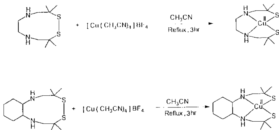
Fig. 27. Synthesis of cis-CuN 2 S 2 complexes by the cleavage of S–S bonding.
