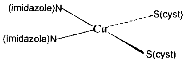
Fig. 4. The proposed Cu A site in cytochrome C oxidase.
