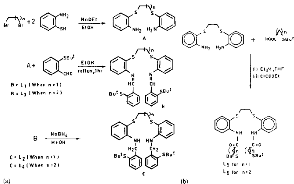
Fig. 21. a) Non-amide hexadentate N_2S_2^*S_2 ( S^* =thioether) donor ligands b) Amide hexadentate N_2S_2^*S_2 ( S^* =thioether) donor ligands c) Non-amide CuN_2S_2^*S_2 complexes d) Amide CuN_2S_2^*S_2 complexes.
