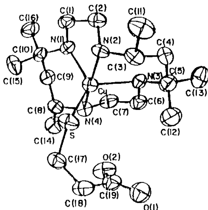
Fig. 9. The structure of [\text{Cu}(\text{tetb})(\text{SCH}_2\text{CH}_2\text{CO}_2)_2] \cdot 2\text{CH}_3\text{OH} .
