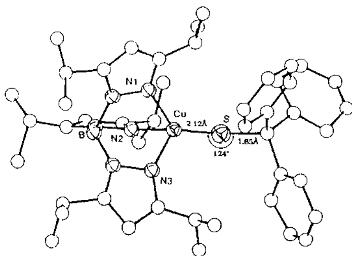
Fig. 13. The structure of [Cu(HB(3,5- i Pr 2 pz) 3 )(SCPh 3 )].
