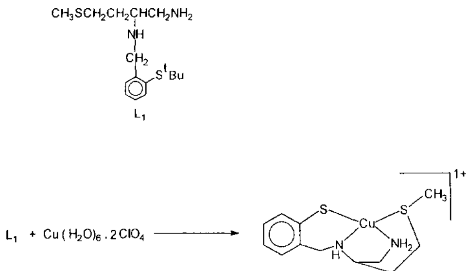
Fig. 20. The \text{CuN}_2\text{S}^*\text{S} ( \text{S}^* = thioether) complex and the ligand.
