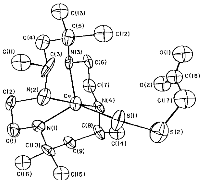
Fig. 10. The structure of [\text{Cu}(\text{tetb})(\text{SSCH}_2\text{CO}_2)] \cdot 2\text{CH}_3\text{OH} .
