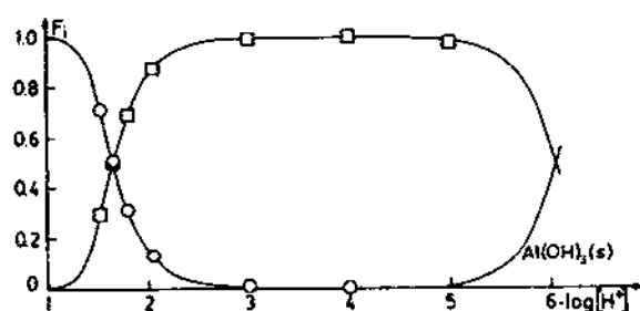
Fig. 8. Fraction of Al(III) in \text{Al}^{3+} ( \circ ) and \text{Al(OH)}_6\text{Mo}_6\text{O}_{19}^{3-} ( \square ) as a function of -\log[\text{H}^+] at B = 0.01 \text{ mol l}^{-1} and C = 0.06 \text{ mol l}^{-1} . —, proposed equilibrium model. Reproduced by permission of American Chemical Society.
