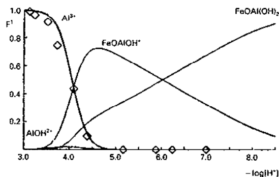
Fig. 9. Distribution diagram showing calculated distribution of aqueous and surface Al complexation. \diamond , total concentration of Al(III) in solution as determined colorimetrically. Reproduced by permission of Elsevier Science Ltd.
