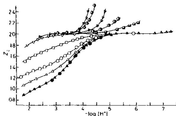
Fig. 2. Part of the experimental data in the \text{H}^+ \text{--} \text{Al}^{3+} –oxalic acid ( \text{H}_2\text{L} ) [31] system plotted as Z_C(-\log [\text{H}^+]) curves. Z_C is defined as the average number of hydroxide ions bound per C. —, calculated from the set of proposed formation constants. Reproduced by permission of The Royal Society of Chemistry, UK.
