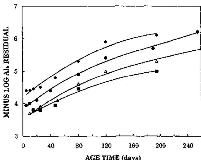
Fig. 4. Disappearance from solution of Al_6 as a function of aging time for aluminum solutions containing various Al:OH ratios: ■, OH:Al = 1.36; △, OH:Al = 2.13; ●, OH:Al = 2.47; ◆, OH:Al = 2.76. From Ref. [10].
