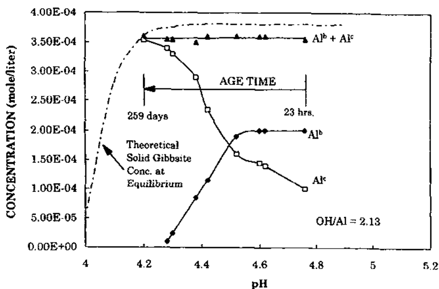
Fig. 3. Concentration of \text{Al}_b and \text{Al}_c as a function of pH and aging time; arrows indicate increasing aging time; total \text{Al(III)} , 4.54 \times 10^{-4} \text{ mol dm}^{-3} ; \text{OH}:\text{Al} = 2.13 . From Ref. [10].
