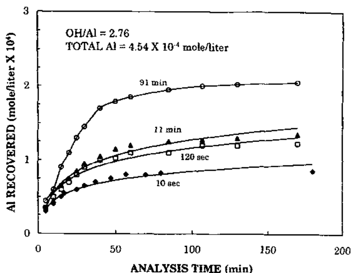
Fig. 2. Effect of length of time of adding base in preparing solutions on the amount of \text{Al}_b formed: total \text{Al(III)} , 4.54 \times 10^{-4} \text{ mol dm}^{-3} ; \text{OH}:\text{Al} = 2.76 . From Refs. [10,14].
