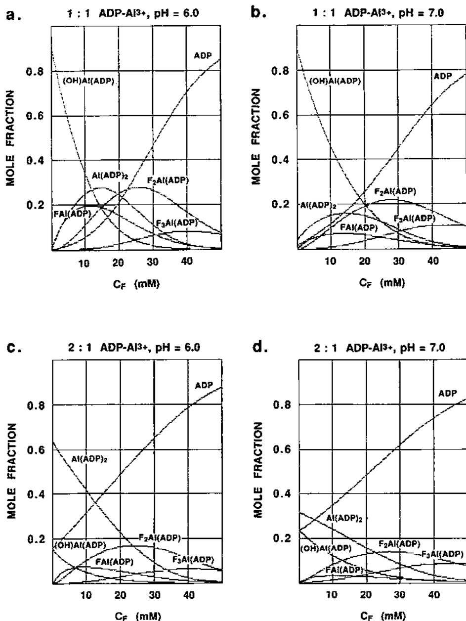
Fig. 5. Species distribution plots on a mole fraction phosphate basis for 1:1 and 2:1 complexes of ADP- Al^{3+} at pH values of 6.0 and 7.0 as a function of total fluoride ion concentration. The four plots presented correspond to the same experimental conditions presented in Fig. 3.
