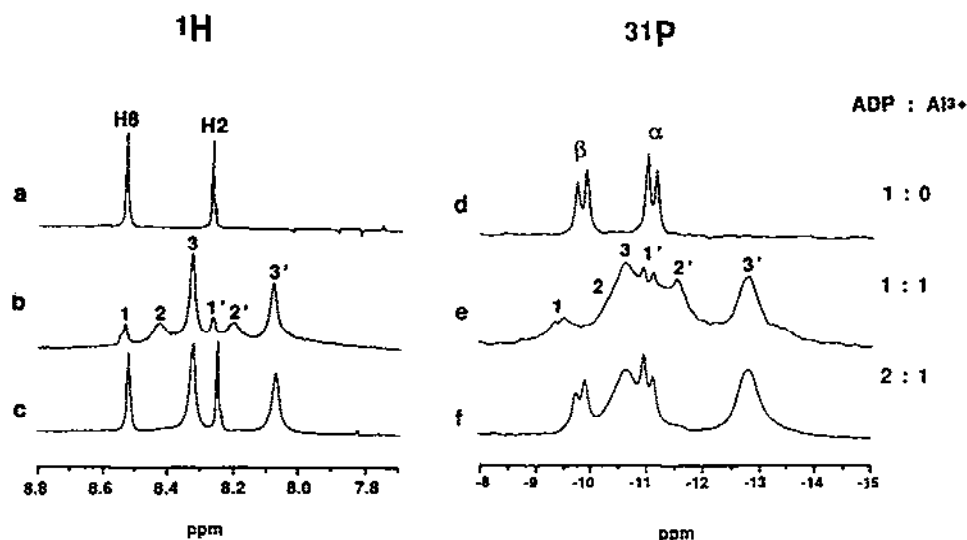
Fig. 2. ^1H (aromatic region) and ^{31}P ( \alpha and \beta phosphate region) NMR spectra of ADP in the absence (spectra a and d) and presence (spectra b, c, e and f) of varying amounts of Al^{3+} at pH 6.0. The concentration of ADP was 10 mM for all spectra except spectra c and f, where the concentration was 20 mM. H8 and H2 in ^1H NMR spectrum a refer to proton positions on the adenine ring. All NMR spectra were acquired at 25°C on a Varian Unity series 300 MHz NMR spectrometer. Spectra were processed using VNMR (version 3.2a) software implemented on a SUN 4-65 computer.
