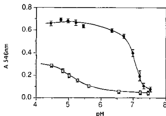
Fig. 1. Variation with pH in absorption at 546 nm of chrome azurol S and \text{Al}^{3+} . Chrome azurol S (20 \mu\text{M} ) + \text{Al}^{3+} (5 \mu\text{M} ) in 1 ml 2 mM Tris acetate buffer pH 4.5 was incubated at room temperature in cuvettes. Aliquots of Tris base (approximately 6 \mu\text{l} aliquots of 0.05 M) were used to raise the pH of the solution in steps up to pH 7, and pH and A_{546} were measured initially and after each addition. Mean values for each pH were calculated from values (from four experiments) varying within 0.1 pH unit. Values in the graph without \text{Al}^{3+} are given after subtraction of a water blank; in those with \text{Al}^{3+} , the value of the dye blank at the appropriate pH has been subtracted: \square , chrome azurol S; \bullet , chrome azurol S + \text{Al}^{3+} .
