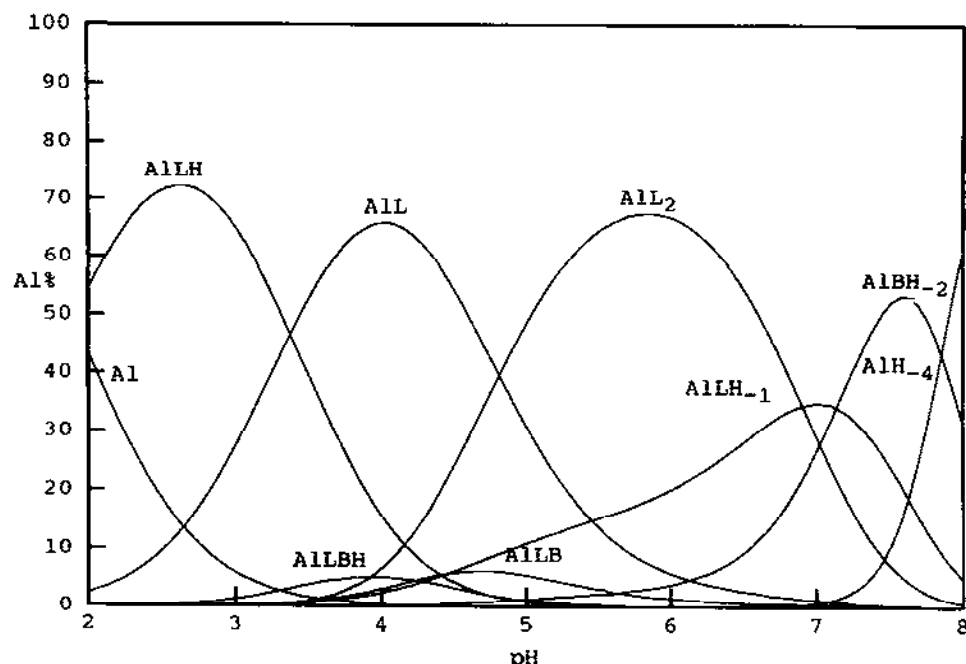
Fig. 4. Species distribution curves for 1 \mu M total Al(III), 1 mM ATP (L) and 1 mM malic acid (B) using log \beta values given in Table 4 and HB, 4.57; H_2B , 7.73; AlBH , 7.34; AlB , 3.8; AlBH_{-1} , 1.32; AlBH_{-2} , -3.74; AlB_2H_{-1} , 4.74; Al_2BH_{-3} , -3.84; AlLBH , 15.52; AlLB , 11.29.
