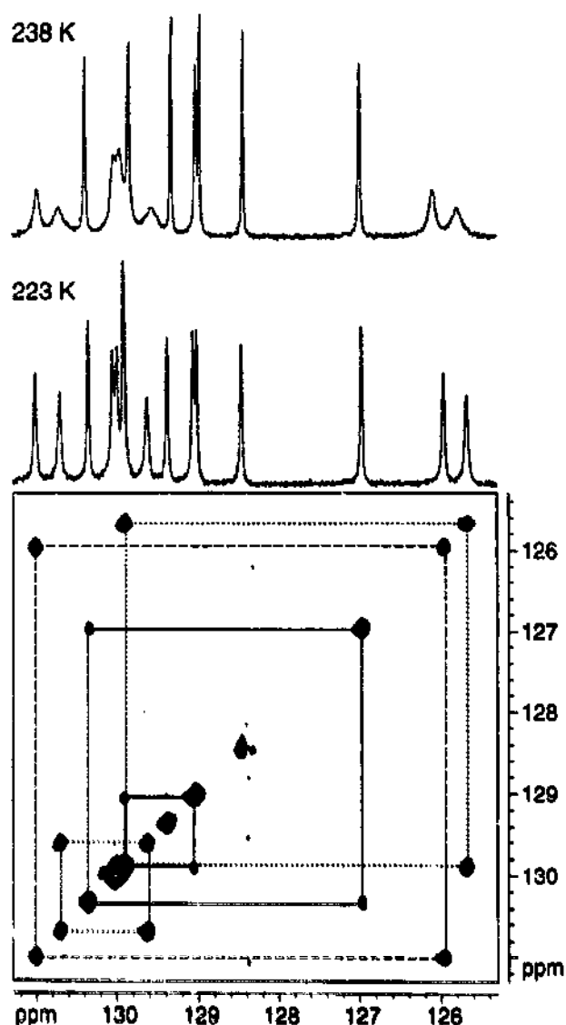
Fig. 2. Contour plot of the aromatic part of the 2-D ^{13}\text{C} exchange spectrum (125.9 MHz) recorded in \text{CDCl}_3 at 223 K showing exchanging ortho - and meta -carbons of the phenyl groups A^{\text{ortho}} (full lines), A^{\text{meta}} (dashed lines) and C^{\text{ortho}} (dotted lines). Top traces are conventional ^{13}\text{C} NMR spectra measured at 223 K (lower) and 238 K (upper).
