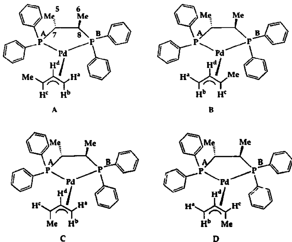
Scheme 3. Four isomers of [\text{Pd}(\eta^3\text{-CH}_3\text{CHCHCH}_3)(\text{S,S-CHIRAPHOS})]\text{CF}_3\text{SO}_3 , 6 .
