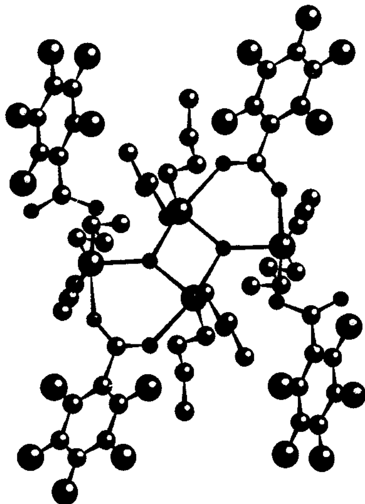
Fig. 4. X-Ray crystal structure of the bis(perfluorobenzoato)tetra- n -butylstannoxane dimer [13].
