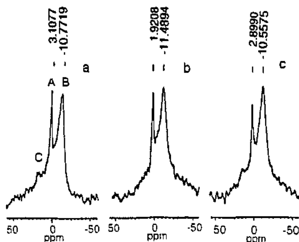
Fig. 2. ^{31}\text{P} NMR spectra (81 MHz) of human erythrocyte membrane ( 15\text{ mg protein ml}^{-1} ) at 37^\circ\text{C} : (a) control, membrane in tris buffer ( 20\text{ mmol l}^{-1} , pH 7.4 and 400\text{ mmol NaCl l}^{-1} ); (b) after 2.5 h incubation; (c) 12 h incubation with cisplatin ( 1.6\text{ mmol l}^{-1} ).
