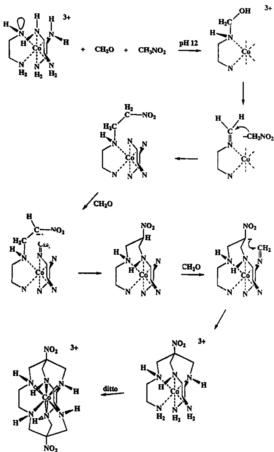
Fig. 2. Template synthesis of [\text{Co}((\text{NO}_2)_2\text{-sar})]^{3+} ion.
