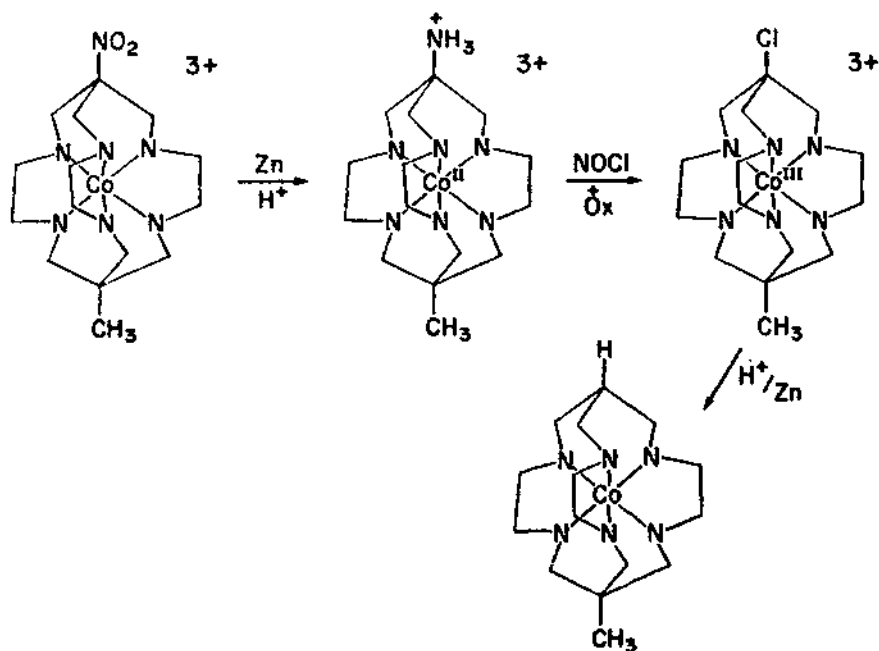
Fig. 3. Variation in substituents for sar-type cages.
