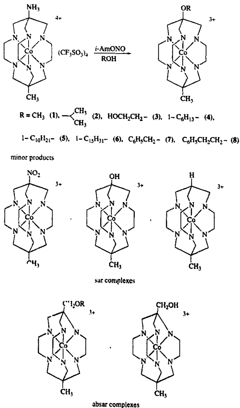
Scheme 1.
