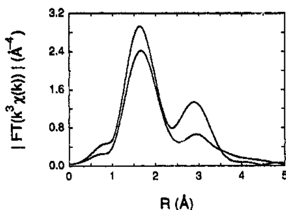
Fig. 4. Fourier transform magnitude of the k^3 -weighted EXAFS at 80 K (Fig. 3) of ferritin reconstituted at 9°C (lower curve) and at 65°C (upper curve). The truncation interval for the Fourier transform extended from k_{\min} = 3.6 \text{ \AA}^{-1} to k_{\max} = 11.3 \text{ \AA}^{-1} . A Hamming window function was used.
