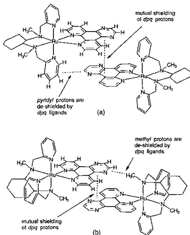
Fig. 8. Representations of possible paired structures formed through \pi - \pi interactions between aromatic bidentate components of (a) rac-cis-α - and (b) rac-cis-β - [\text{Ru}(\text{picchxnMe}_3)(\text{dpq})]^{2+} species. An interpretation of the consequent magnetic shielding effects observed in ^1\text{H} NMR spectra is given.
