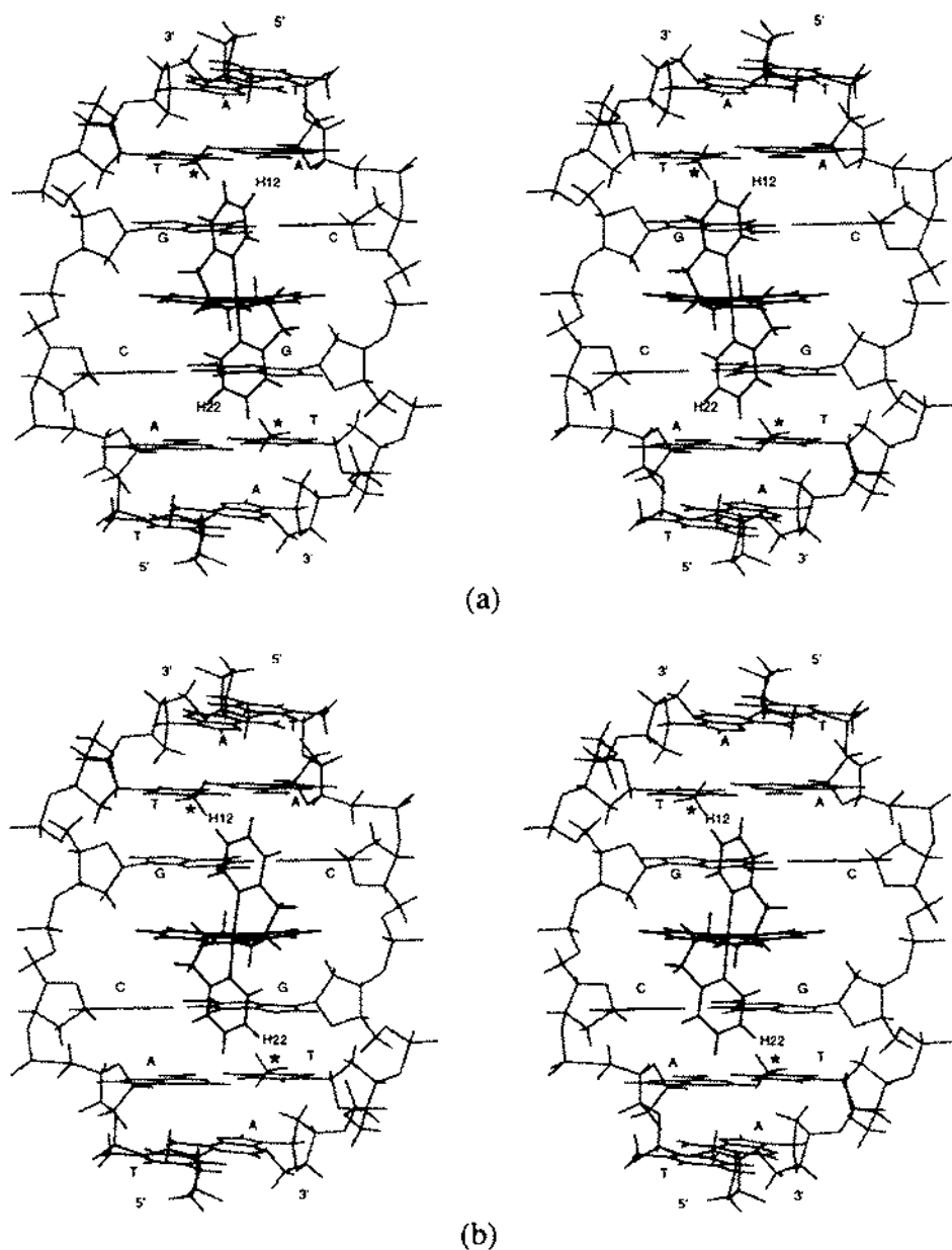
Fig. 9. Stereoscopic views of (a) the A\text{-}\alpha\text{-} and (b) the A\text{-}\alpha\text{-} enantiomeric forms of a \text{cis-2-[Ru(picen)(bidentate)]}^+ cation positioned for intercalation into a fixed model \text{d(TACGTA)}_2 duplex fragment [11]. The A enantiomer shows a steric interaction between the pyridyl protons H12 and H22 of the picen ligand and the thymine methyl groups (indicated *) in the major groove of the duplex. Steric bulk or secondary binding components incorporated into the tetradentate in these positions should result in a major enhancement of the enantioselective and sequence recognition capabilities of metallointercalators of this type.
