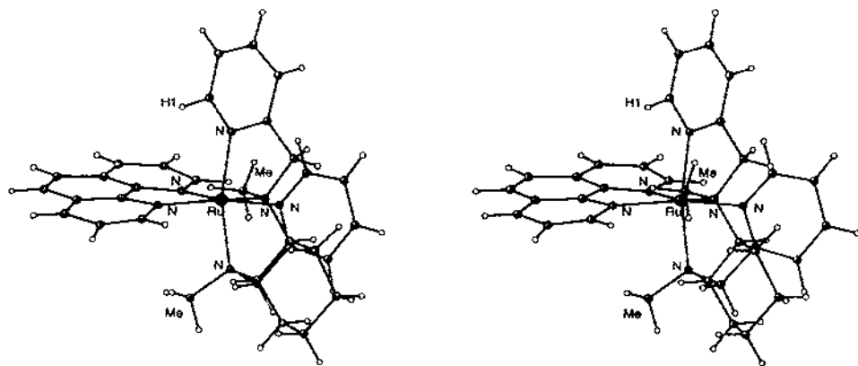
Fig. 7. A stereoview [110] of the molecular structure of the cis-A-β -[Ru(SS-piechxnMe 2 )(phen)] 2+ cation [75, 102] derived from the crystal structure of its enantiomer [104]. A comparison with the structure of the RR -piechxn diastereoisomer shown in Fig. 5 illustrates topological changes resulting from N -methylation of the tetradentate. Primary steric contacts made with DNA by metallointercalators based on this geometry would involve the lower methyl group and the \alpha -pyridyl proton H1.
