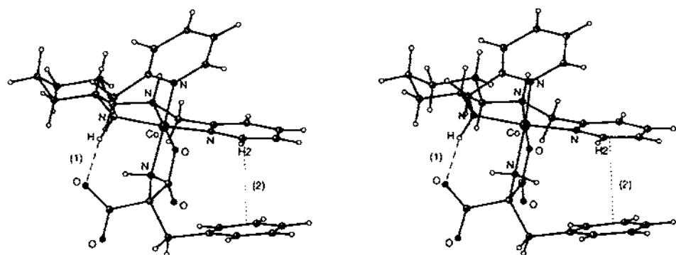
Fig. 1. A stereoview [110] of the molecular structure of the A\text{-}\beta_1\text{-[Co(RR-picchn)(R-ABMA)]}^+ cation (atomic coordinates obtained from crystallographic data [8]). The two favourable noncovalent interactions indicated between the picchn and ABMA ligands are (1) a hydrogen bond involving the amine NH and unbound carboxylate group, and (2) \pi -stacking of the aromatic pyridyl and phenyl ring components. A close structural relationship exists with that shown Fig. 2.
