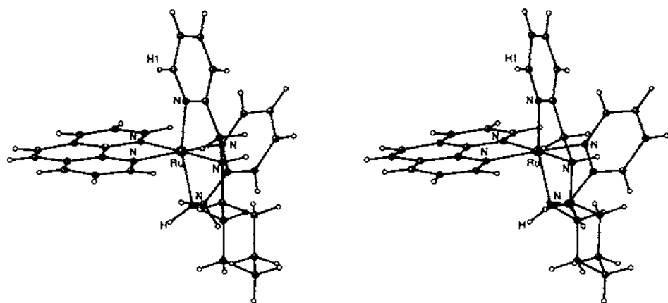
Fig. 5. A stereoview [11] of the molecular structure of the A- \beta -[Ru(RR-picchxn)(phen)] 2+ diastereoisomer (atomic coordinates obtained from crystallographic data [104]). Note the interchange of the positions in the coordination sphere of a pyridyl and an amine group of the tetradentate in comparison with a cis-α stereoisomer (Fig. 4). The lower amine group would provide the opportunity of nucleobase sequence selectivity through H-bonding for metal-lointercalators based on this structure.
