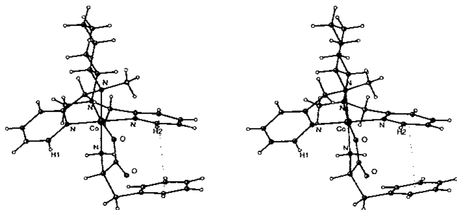
Fig. 3. A stereoview [110] of the molecular structure of the A - \alpha -[Co(SS-picchxnMe 2 )( S -phe)] 2+ cation (atomic coordinates obtained from crystallographic data [11]). A favourable \pi -stacking interaction between one pyridyl ring of SS -picchxnMe 2 and the phenyl substituent of the S -phe aminoacidate ligand is indicated. The structure may be related to diagram (IV(c)).
