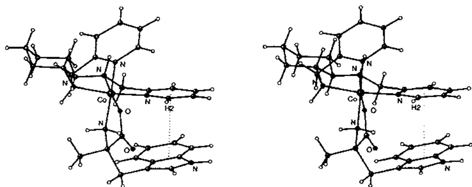
Fig. 2. A stereoview [110] of the molecular structure of the A\text{-}\beta_1\text{-[Co(RR-picchn)(S-}\alpha\text{-Me-trp)]}^{2+} cation (atomic coordinates obtained from crystallographic data [10]). A favourable \pi -stacking interaction between one pyridyl ring of RR -picchn and the aromatic indole substituent of the S -aminoacidate ligand is indicated. The structure may be related to diagram (IV(e)).
