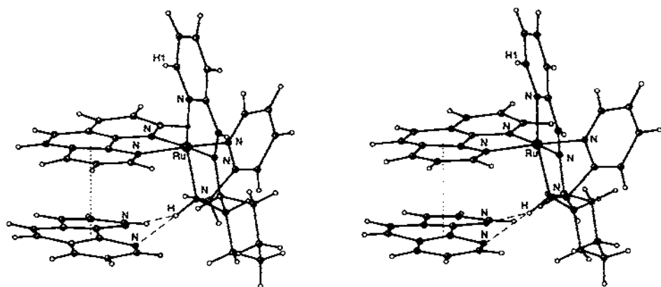
Fig. 6. A stereoview [110] of the molecular structure of the A\text{-}\beta\text{-[Ru(RR-picchxnmi)(phen)]}^{2+} phen solvate complex obtained after photo-oxidation of the corresponding picchxn species [54,56] shown in Fig. 5. Atomic coordinates were obtained from crystallographic data [104]. Favourable intermolecular \pi -stacking and H-bonding interactions between the cation and the free heterocyclic base are indicated.
