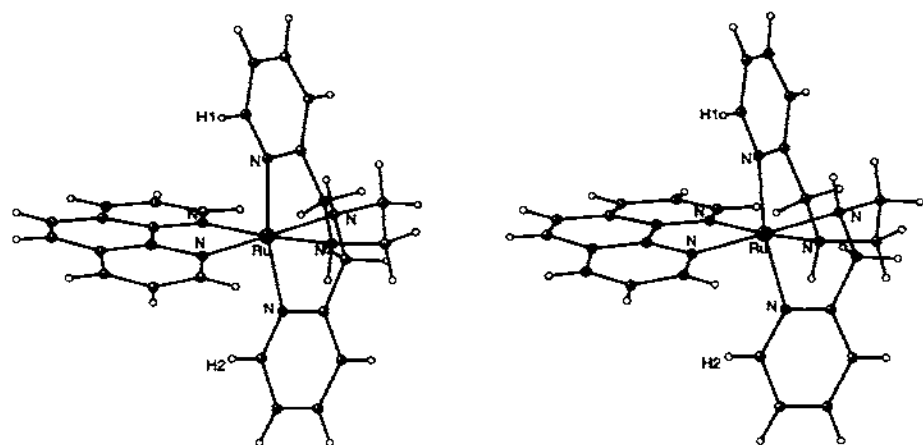
Fig. 4. A stereoview [110] of the molecular structure of the A enantiomer of cis-α -[Ru(picen)(phen)] 2+ (atomic coordinates obtained from crystallographic data [104]). The molecule has C 2 symmetry and hence the stereochemical environments above and below the phen moiety, exemplified by \alpha -pyridyl protons H1 and H2, are equivalent. These protons would make primary steric contacts with duplex DNA for metal-lointercalators based on this geometry.
