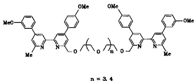
Fig. 19. Structure of bipyridyl capped polyethers.
