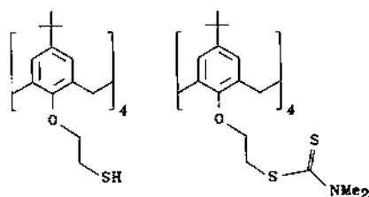
Fig. 48. Thiol and dithiocarbamoyl derivatized calix[4]arenes.
