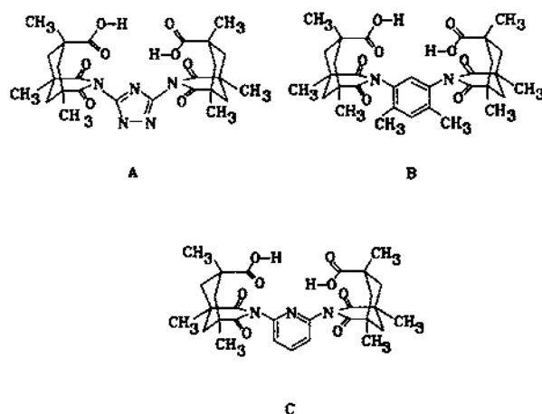
Fig. 23. Structures of multidentate N, O chelates.
