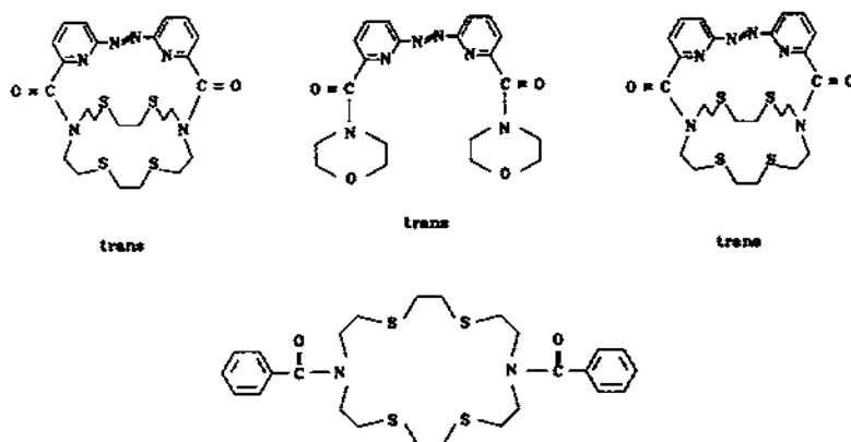
Fig. 28. Structures of thiacycrown complexes.
