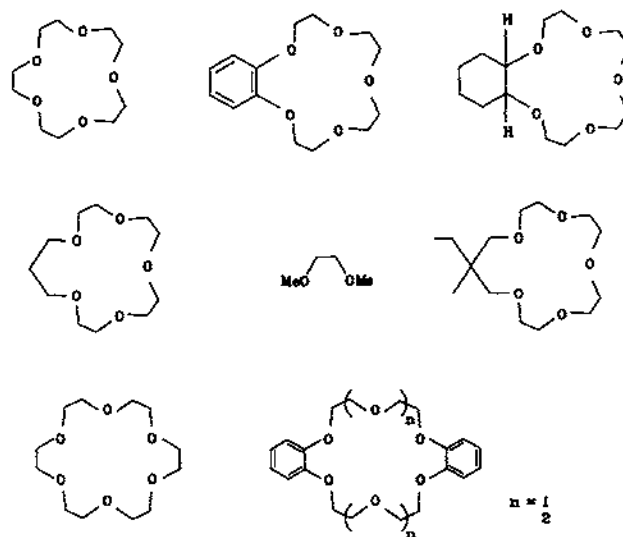
Fig. 35. Structures of crown ethers.
