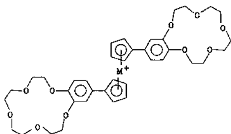
Fig. 44. Structure of metallocene-substituted crown ethers.
