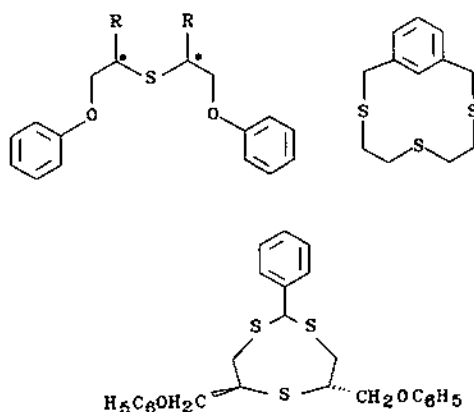
Fig. 41. Structures of thiacycrown ethers.
