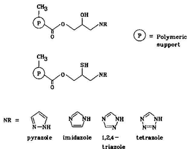
Fig. 9. Polymer-bound azoles.
