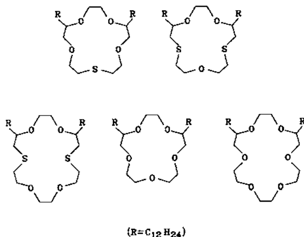
Fig. 45. Structures of crown and thiocrown ethers.
