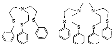
Fig. 20. Structures of O, S and N, S chelates.
