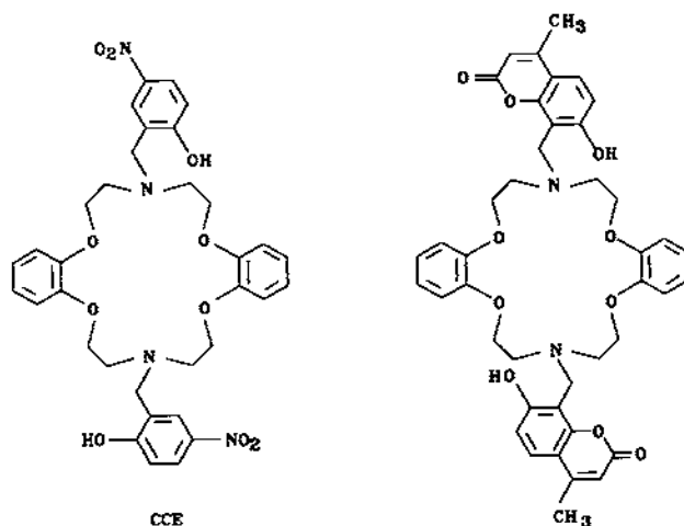
Fig. 33. Structures of chromogenic and fluorogenic crown ethers.
