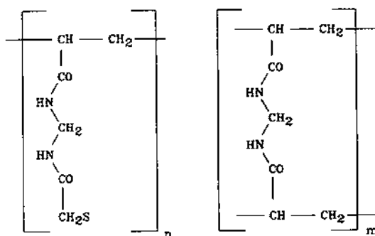
Fig. 26. Structures of derivatized resins.
