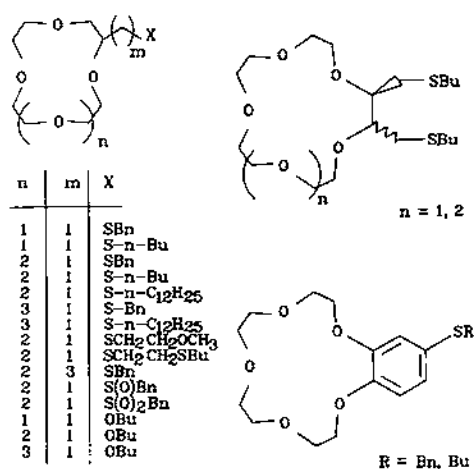
Fig. 42. Structures of thiolariat ethers.
