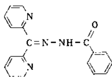
Fig. 13. Structures of DPKSH and DPKBH.
