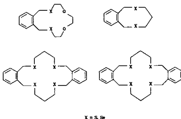
Fig. 37. Structures of thiacycrocrown and selenocycrocrown ethers.
