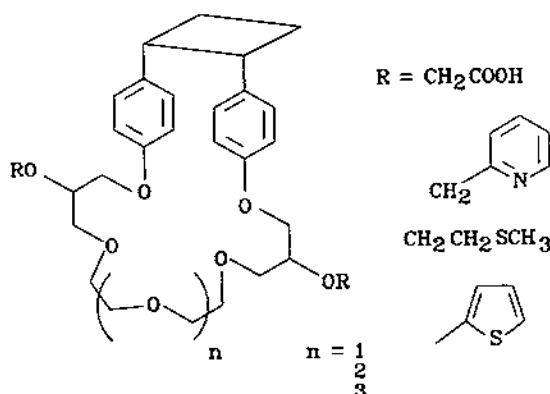
Fig. 32. Structures of crownophanes.
