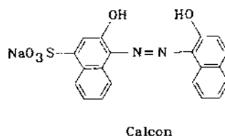
Fig. 5. Structure of Calcon.
