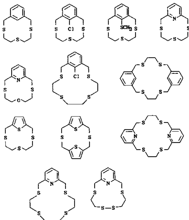
Fig. 43. Structures of thiacyanines.
