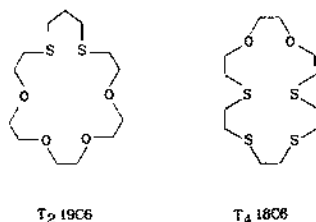
Fig. 39. Structures of T219C6 and T418C6.
