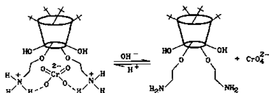
Fig. 50. Proton-switchable calix[4]arene extractant for Cr(VI).
