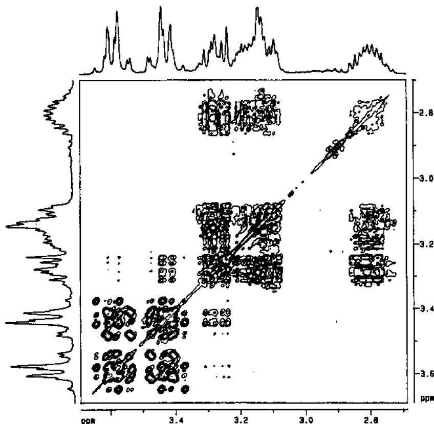
Fig. 6. Magnitude COSY spectrum of [\text{Co}(\text{cee})(\text{NO}_2)_2]\text{Cl} .
