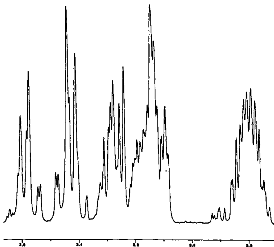
Fig. 3. Proton spectrum of [\text{Co}(\text{eee})(\text{NO}_2)_2]\text{Cl} .
