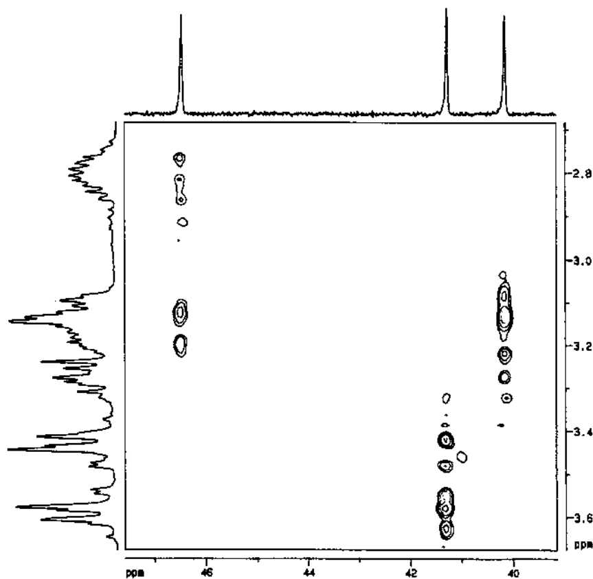
Fig. 4. HETCOR spectrum of [\text{Co}(\text{III})(\text{NO}_3)_2]\text{Cl} .
