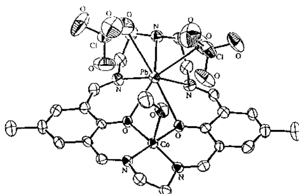
[\text{CoPb}(\text{L}^6)(\text{MeOH})(\text{ClO}_4)_2]
