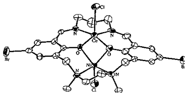
[CuNi(L 8 )Cl 2 ]
