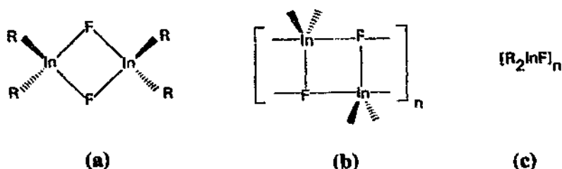
Fig. 18. Degree of aggregation for diorganoindium fluorides in solution: (a) \text{R} = \text{CH}_2\text{Ph} [21], Mes [21]; (b) \text{R} = ^i\text{Pr} [20]; (c) \text{R} = \text{Me} [76], Et [79].
