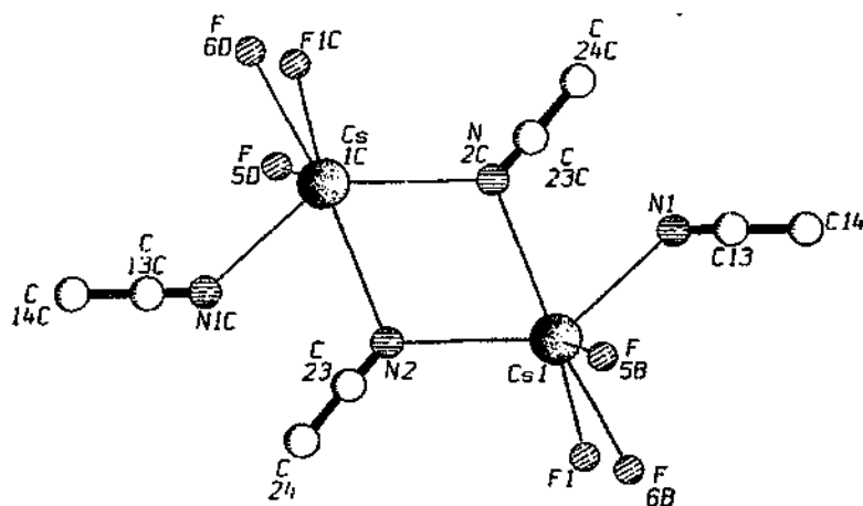
Fig. 22. Centrosymmetric dimer formed by \text{Cs}^+ ions and acetonitrile molecules in [(\text{Pr})_2\text{InF}]_3\{\text{CsF} \cdot 2\text{MeCN}\} . The complete coordination sphere of the caesium cations is shown (SCHAKAL [29]).
