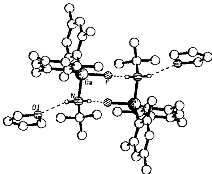
Fig. 15. Centrosymmetric dimer of [\text{Mes}_2\text{Ga}(\text{F})\text{NH}_2(\text{'Bu})] in [\text{Mes}_2\text{Ga}(\text{F})\text{NH}_2(\text{'Bu})]\cdot 2.5\text{THF} (SCHAKAL [29]).
