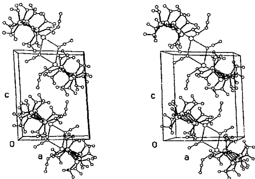
Fig. 23. Stereoscopic view of the unit cell of \{[(i\text{Pr})_2\text{InF}]_3[\text{CsF} \cdot 2\text{MeCN}]\} along the b axis.
