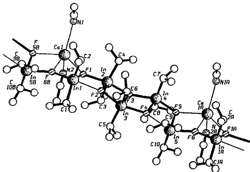
Fig. 21. Part of the polymeric chain of [(\text{Pr})_2\text{InF}]_3\{\text{CsF} \cdot 2\text{MeCN}\} (SCHAKAL [29]).
