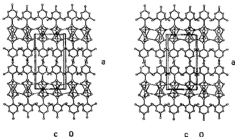
Fig. 8. Stereoscopic view of the unit cell of \text{Cs[MesGaF}_3\text{]} parallel to (100) (ORTEP [65]).
