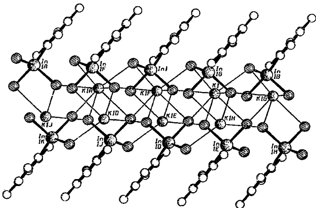
Fig. 27. Part of one layer in K[MesInBr_3] (SCHAKAL [29]).
