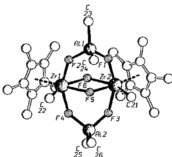
Fig. 4. Plot of one of the crystallographically independent molecules [\text{Cp}^*(\text{Me})\text{ZrF}_3\text{AlMe}_2]_2 (SCAKAL [29]).
