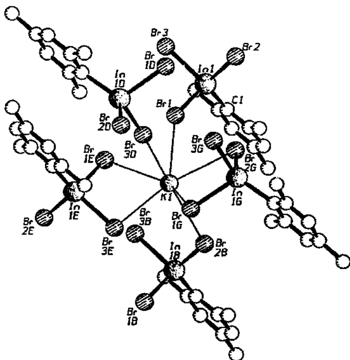
Fig. 26. Coordination sphere of the K^+ ion in K[\text{MesInBr}_3] (SCHAKAL [29]).
