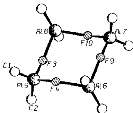
Fig. 1. Computer-generated plot of [\text{Me}_2\text{AlF}]_4 (SCHAKAL [29]) according to gas phase electron diffraction.
