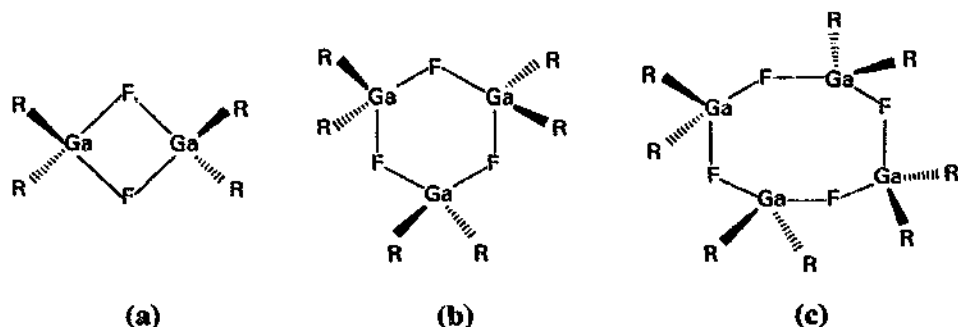
Fig. 6. Degree of aggregation for diorganogallium fluorides in solution: (a) \text{R} = \text{CH}_2\text{Ph} [17], \text{Mes} [17]; (b) \text{R} = \text{Me} [63], \text{Et} [63], {}^i\text{Pr} [17]; (c) \text{R} = \text{Me} [64].
