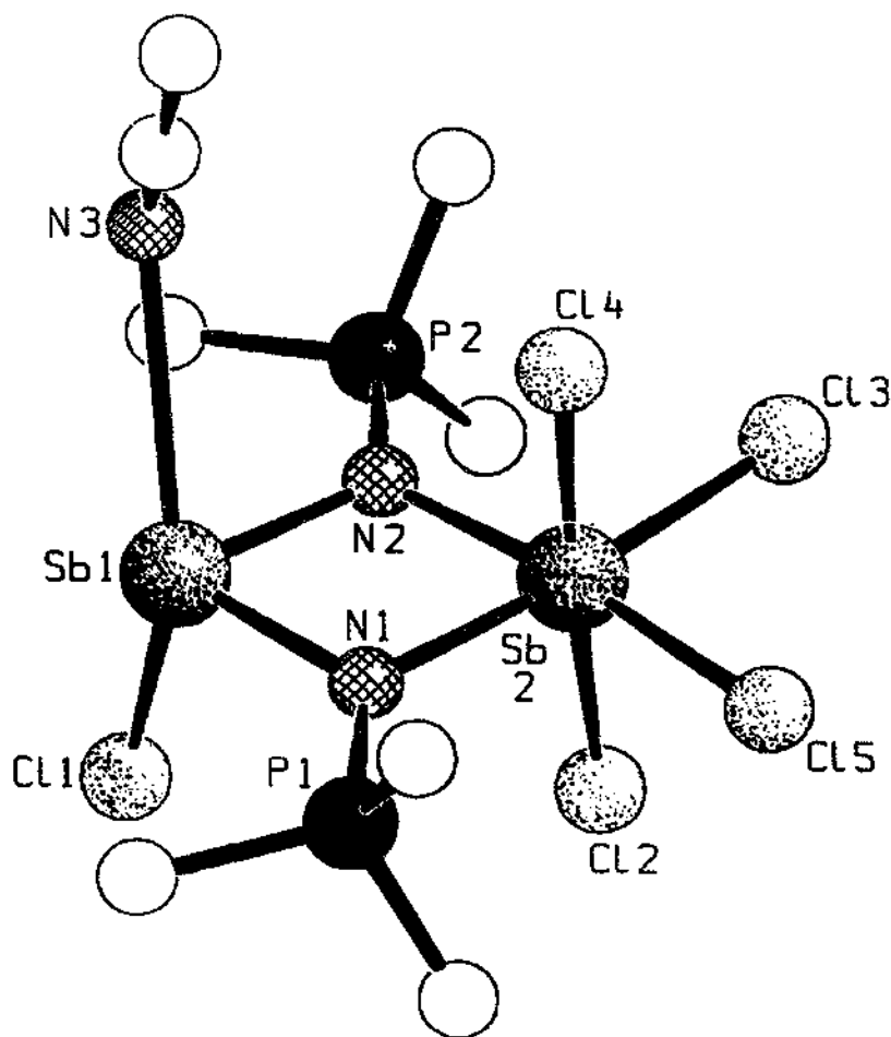
Fig. 26. View of the cation [\text{ClSb}(\text{NPMe}_3)_2\text{SbCl}_4(\text{CH}_3\text{CN})]^+ in the structure of [\text{ClSb}(\text{NPMe}_3)_2\text{SbCl}_4(\text{CH}_3\text{CN})]\text{SbCl}_6 .
