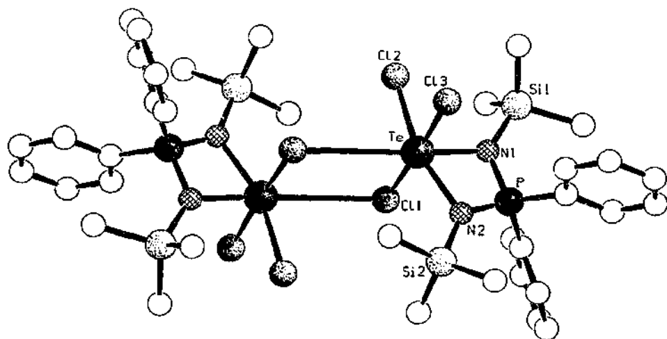
Fig. 56. Molecular structure of [\text{Ph}_3\text{P}(\text{NSiMe}_3)_2\text{TeCl}_3]_2 .
