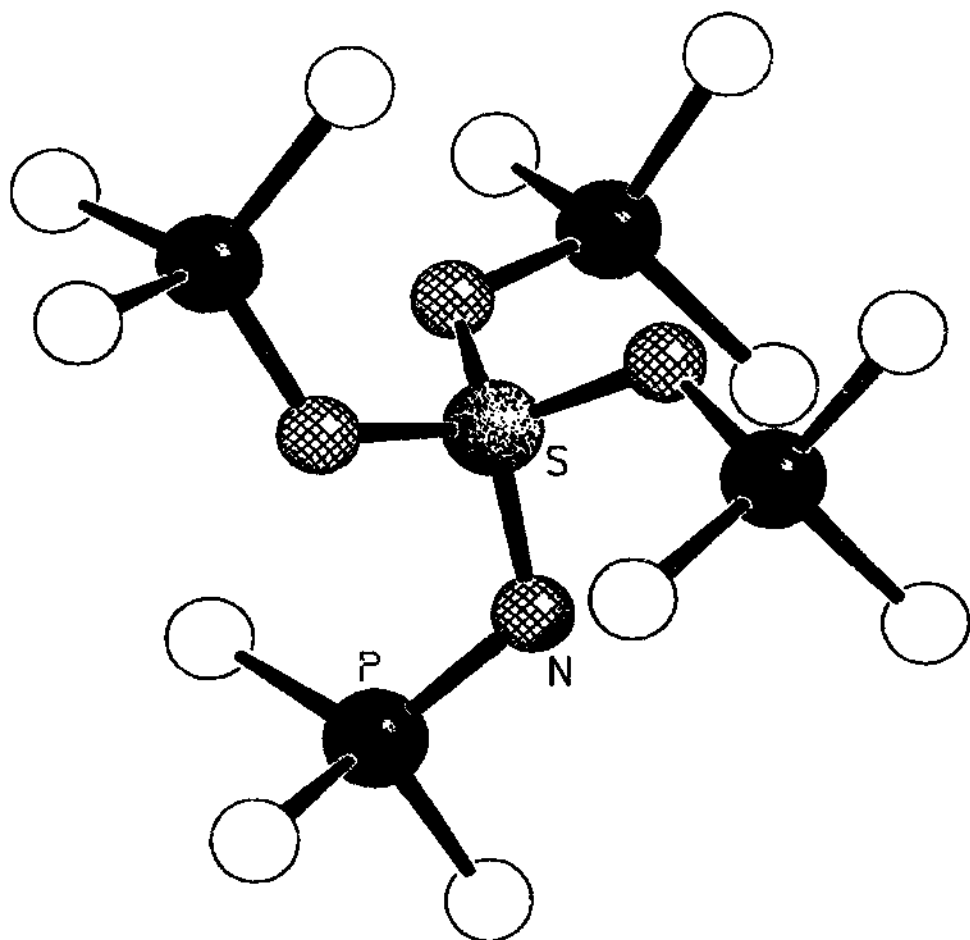
Fig. 38. View of the dication [S(NPM 3 ) 4 ] 2+ in the structure of [S(NPM 3 ) 4 ] 2 Cl 2 ·4CH 3 CN.
