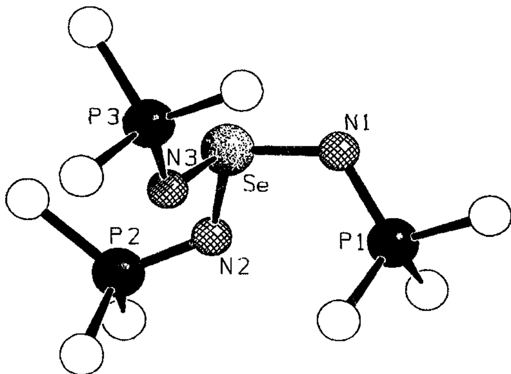
Fig. 51. View of the cation [\text{Se}(\text{NPM}_3)_3]^+ in the structure of [\text{Se}(\text{NPM}_3)_3]\text{Cl} \cdot \text{C}_7\text{H}_8 .
