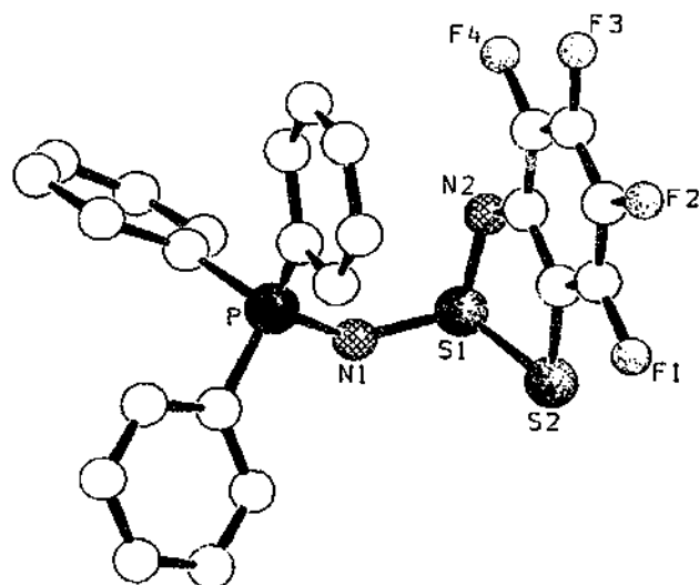
Fig. 34. Molecular structure of \text{Ph}_3\text{PN}(\text{S}_2\text{NC}_6\text{F}_4) .
