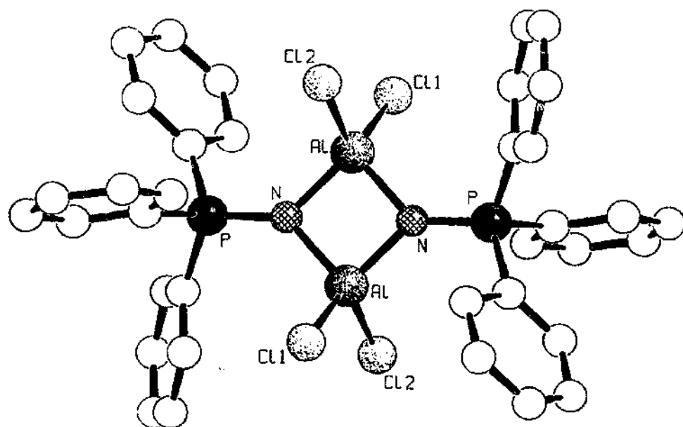
Fig. 3. Molecular structure of [\text{Cl}_2\text{Al}(\text{NPPh}_3)]_2 .
