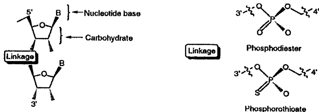
Fig. 3. Modified nucleotides.
