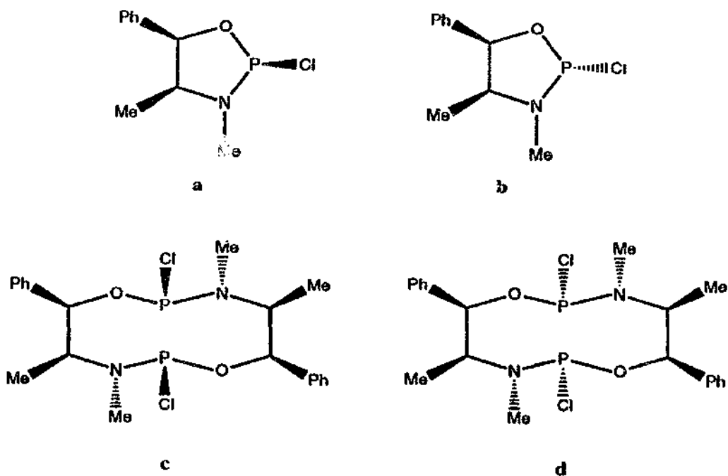
Fig. 9. Possible monomeric and dimeric forms of the chiral 2-chloro-1,3,2-oxazaphospholidine derived from (1 R ,2 S )-ephedrine.
