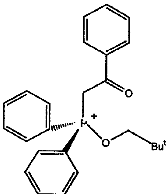
Fig. 5. Structure of neopentyloxy(phenacyl)diphenylphosphonium bromide (anion omitted for clarity).
