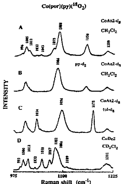
Fig. 13. Resonance Raman spectra of ^{18}\text{O}_2 adducts of Co(porphyrin)(py) complexes (excitation at 406.7 nm): (A) CoAz2- \text{d}_8 , \text{CH}_2\text{Cl}_2 ; (B) CoAz2- \text{d}_8 , \text{CH}_2\text{Cl}_2 ; (C) CoAz2- \text{d}_8 , \text{tol-}\text{d}_8 ; (D) CoDe2, \text{CD}_2\text{Cl}_2 (from Ref. [61]).
