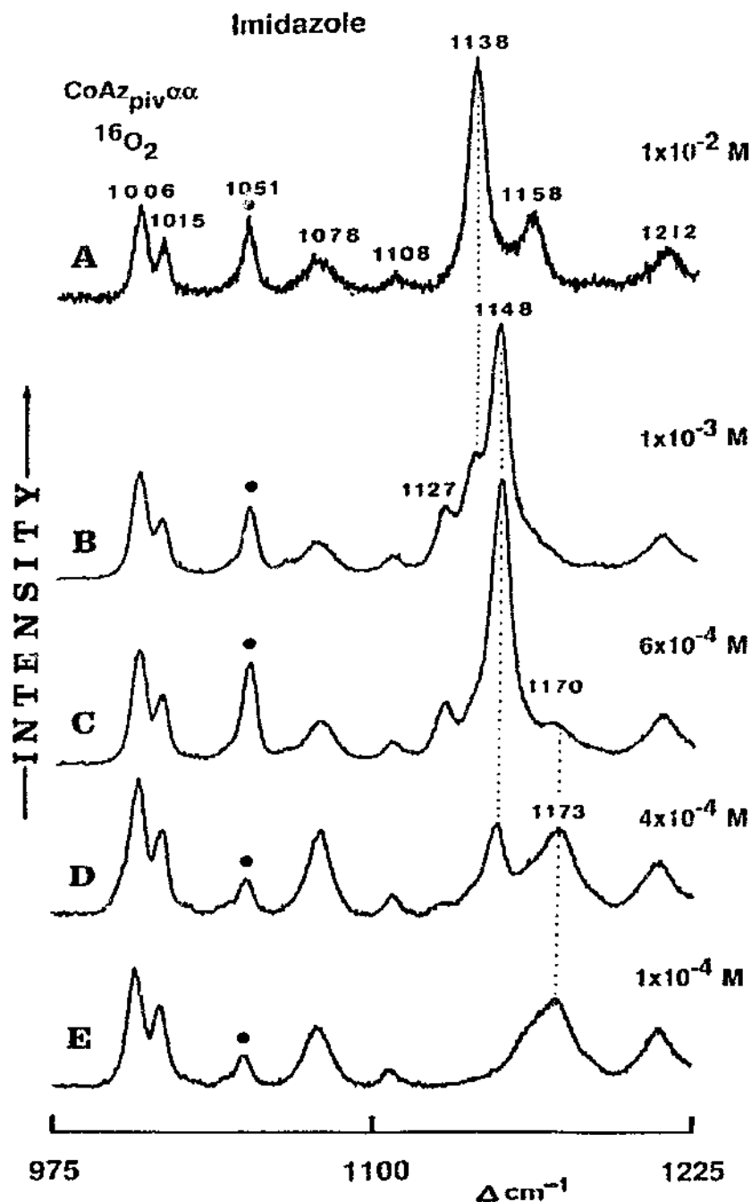
Fig. 10. Influence of imidazole concentration on resonance Raman spectra of the 16 O 2 adduct of CoAz piv αα complex with imidazole. Temperature at ~185 K. Spectral conditions as in Fig. 8 (from Ref. [77]).
