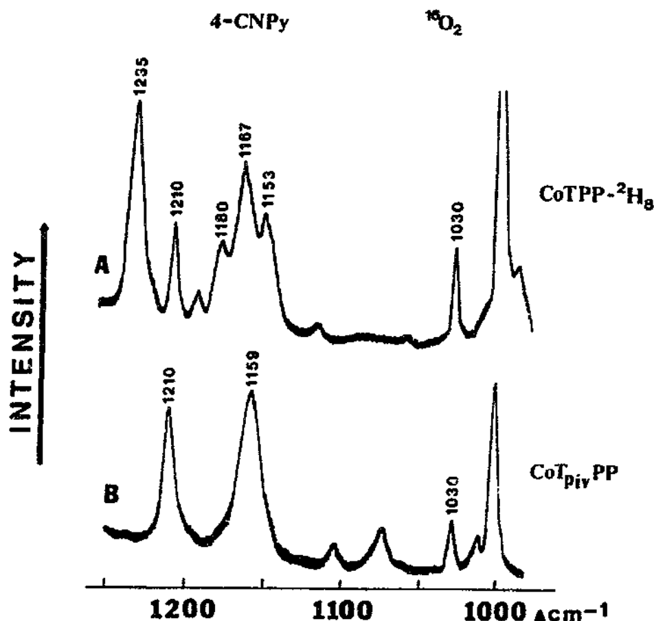
Fig. 17. Resonance Raman spectra of \text{Co(TPP-}^2\text{H}_8\text{)} (trace A) and \alpha^1\text{-Co(TpivPP)} (trace B) in toluene containing 3% 4-cyanopyridine at -85^\circ\text{C} under \sim 4 atm of ^{16}\text{O}_2 pressure (from Ref. [84]).
