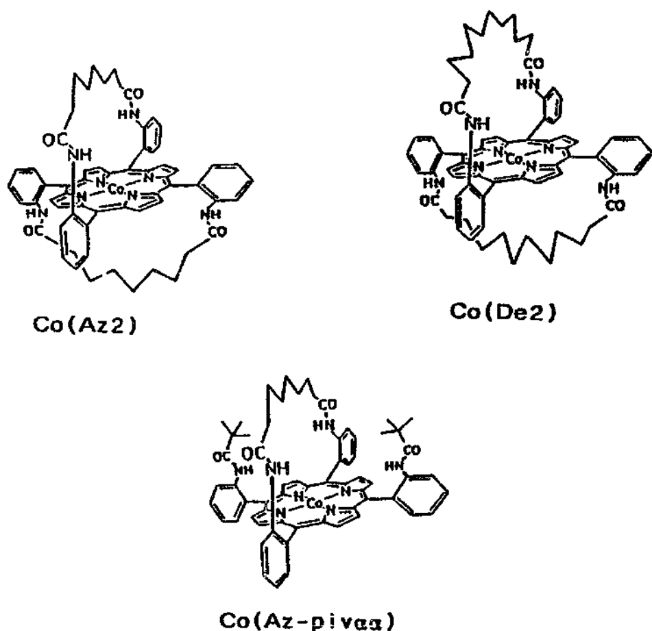
Fig. 12. Structures of Co(Az2), Co(De2) and Co(Az-pivaa).
