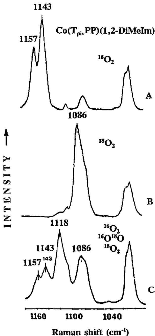
Fig. 4. Resonance Raman spectra (406.7-nm excitation) of dioxygen adducts of \text{Co}(\text{T}_{\text{piv}}\text{PP}) in \text{CH}_2\text{Cl}_2 containing 3% of 1,2-dimethylimidazole at -90^\circ\text{C} under ca. 4 atm. of \text{O}_2 pressure: (A) ^{16}\text{O}_2 ; (B) ^{18}\text{O}_2 ; (C) ^{16}\text{O}_2/^{16}\text{O}^{18}\text{O}/^{18}\text{O}_2 = 1/2/1 (adapted from Ref. [60]).
