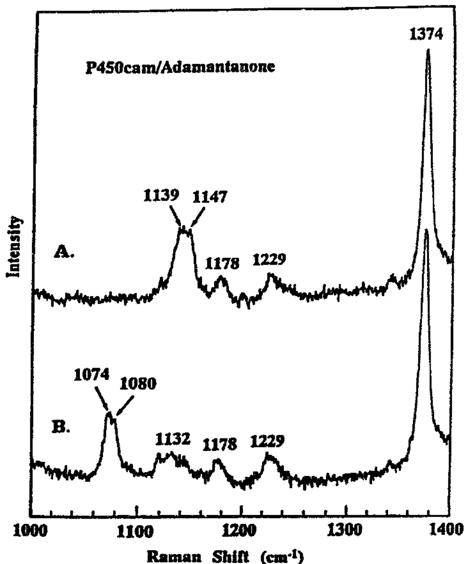
Fig. 20. Resonance Raman spectra of dioxygen adduct of adamantanone-bound cytochrome P450 cam at -80^{\circ}\text{C} in the \nu(\text{O}-\text{O}) region: trace A, ^{16}\text{O}_2 ; trace B, ^{18}\text{O}_2 . Excitation at 413.1 nm (from Ref. [96]).
