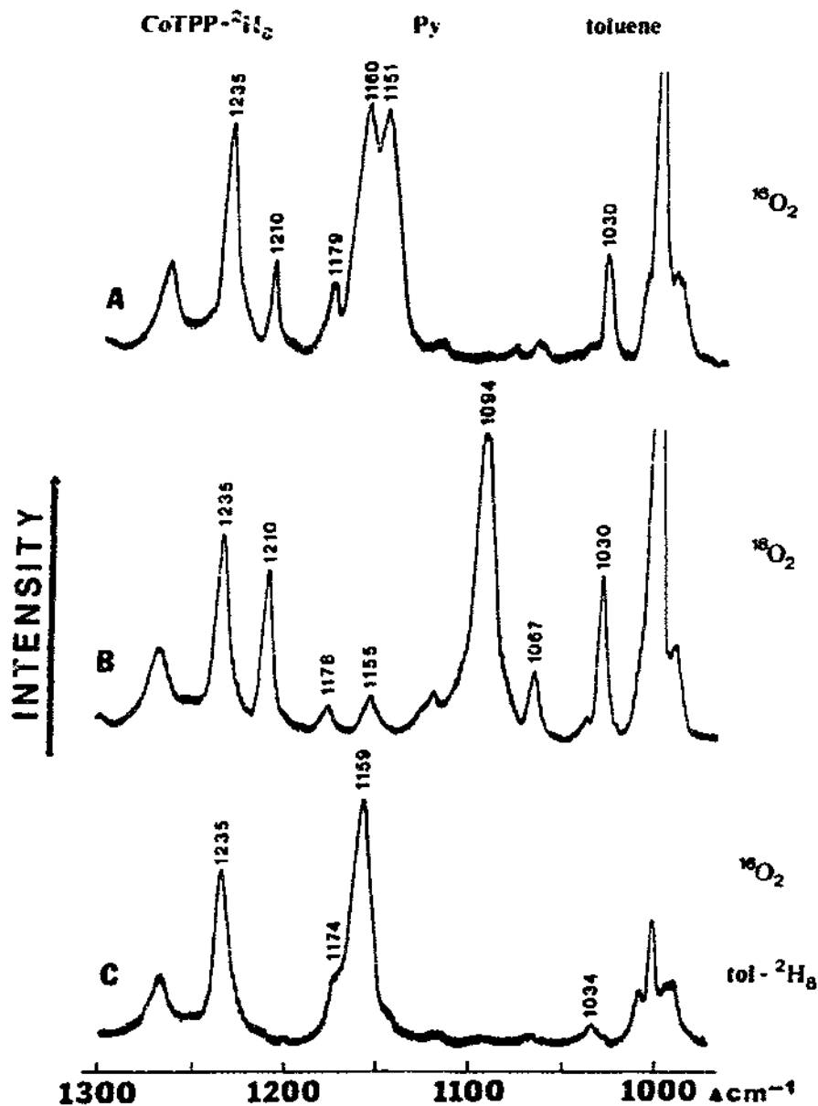
Fig. 15. Resonance Raman spectra of \text{Co(TPP-}^2\text{H}_8\text{)} in toluene containing 3% pyridine at -85^\circ\text{C} under \sim 4 atm of \text{O}_2 pressure: (A) ^{16}\text{O}_2 ; (B) ^{18}\text{O}_2 ; (C) ^{16}\text{O}_2 , toluene- ^2\text{H}_8 (from Ref. [84]).
