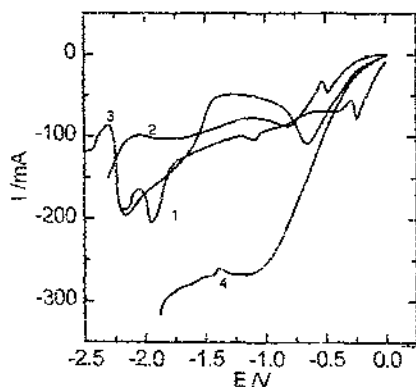
Fig. 9. Voltammetric curves in the \text{K}_2\text{TiF}_6 -KCl system. (1) \text{K}_2\text{TiF}_6 ; (2) \text{K}_2\text{TiF}_6 + 5 mol% KCl; (3) \text{K}_2\text{TiF}_6 + 50 mol% KCl; (4) \text{K}_2\text{TiF}_6 + 90 mol% KCl.
