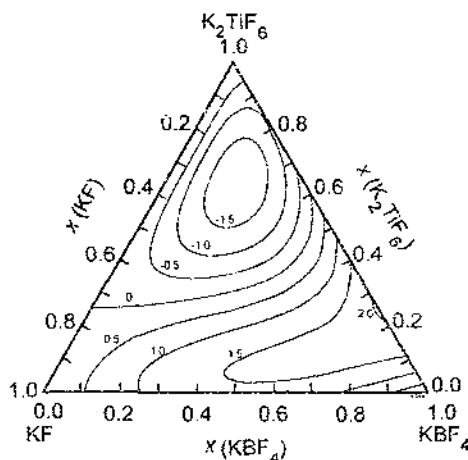
Fig. 24. Excess molar volume of the \text{KF}-\text{KBF}_4-\text{K}_2\text{TiF}_6 system at T=1100\text{ K} . Values are in \text{cm}^3\text{ mol}^{-1} .
