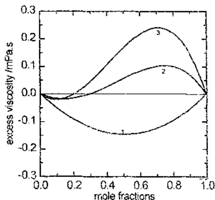
Fig. 17. Excess viscosity of the boundary binary systems at T = 1100 K. (1) KF-KCl; (2) KCl- K_2TiF_6 ; (3) KF- K_2TiF_6 .
