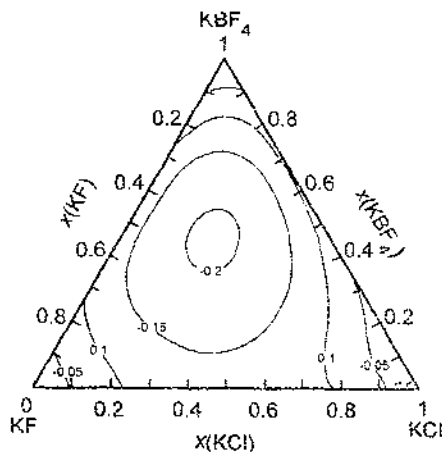
Fig. 13. Excess viscosity of the \text{KF}-\text{KCl}-\text{KBF}_4 system at T=1100\text{ K} . Values are in \text{mPa}\cdot\text{s} .
