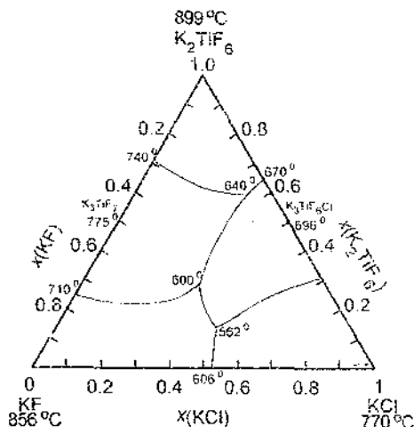
Fig. 15. Phase diagram of the \text{Kf}-\text{KCl}-\text{K}_2\text{TiF}_6 system.
