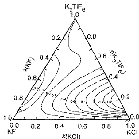
Fig. 16. Excess molar volume of the KF–KCl– K_2TiF_6 system at T = 1100 K. Values are in cm^3 mol^{-1} .
