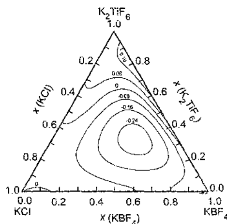
Fig. 32. Excess viscosity of the \text{KCl}-\text{KBF}_4-\text{K}_2\text{TiF}_6 system at T = 1100\text{ K} . Values are in \text{mPa.s} .
