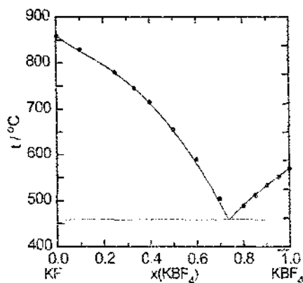
Fig. 21. Phase diagram of the \text{KF}-\text{KBF}_4 system.
