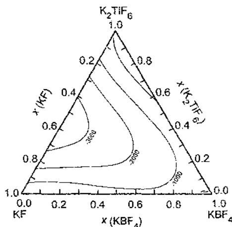
Fig. 20. Excess Gibbs' energy of mixing in the \text{KF}-\text{KBF}_4-\text{K}_2\text{TiF}_6 system. Values are in \text{J mol}^{-1} .
