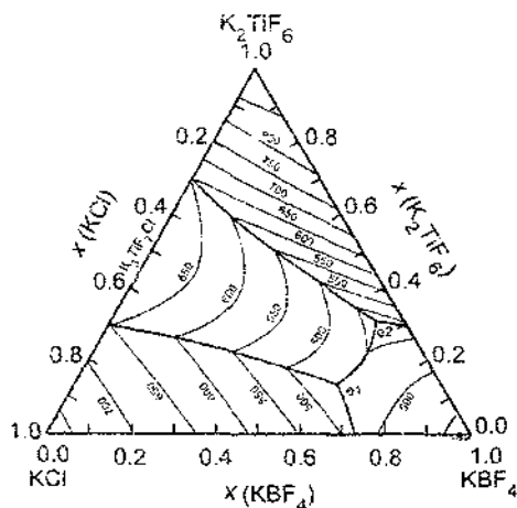
Fig. 26. Phase diagram of the \text{KCl}-\text{KBF}_4-\text{K}_2\text{TiF}_6 system.
