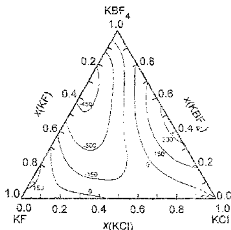
Fig. 10. Excess Gibbs' energy of mixing in the KF-KCl-KBF 4 system. \Delta G^E values are in J mol -1 .
