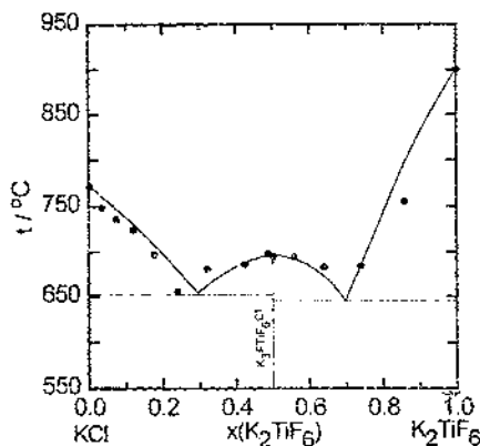
Fig. 29. Phase diagram of the KCl–K 2 TiF 6 system.
