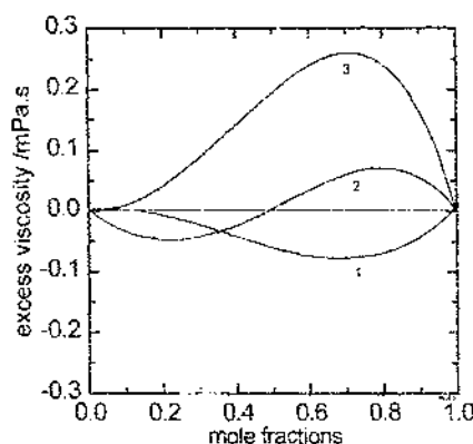
Fig. 33. Excess viscosity of the boundary binary system at T = 1100\text{ K} . (1) \text{KCl}-\text{KBF}_4 ; (2) \text{KCl}-\text{K}_2\text{TiF}_6 ; (3) \text{KBF}_4-\text{K}_2\text{TiF}_6 .
