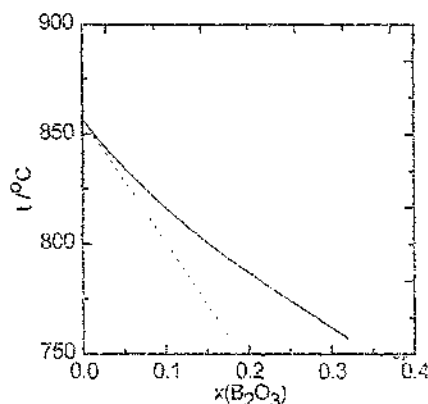
Fig. 3. Liquidus curve of KF in the KF-B 2 O 3 system. Patarek et al. [35] (—); Chrenkova and Daneš [38] (---); limiting course for two new particles (---).
