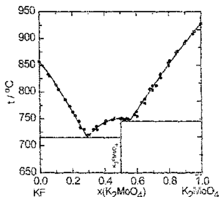
Fig. 2. Phase diagram of the KF– K_2MoO_4 system. Experiment [34,35] (●); calculated (○).
