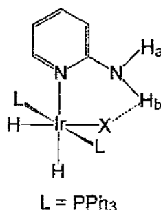
Fig. 4. This class of iridium complexes were used to estimate hydrogen bond strengths ( Ir \cdots X \cdots HN ) by measuring the barrier to rotation about the C–N bond. The barrier was measured by NMR lineshape analysis of the coalescence of H_a and H_b .
