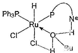
Fig. 6. A hydrogen bond to chloride was proposed in this t BuOH adduct although hydrogen bonding to a hydride ligand is equally possible.
