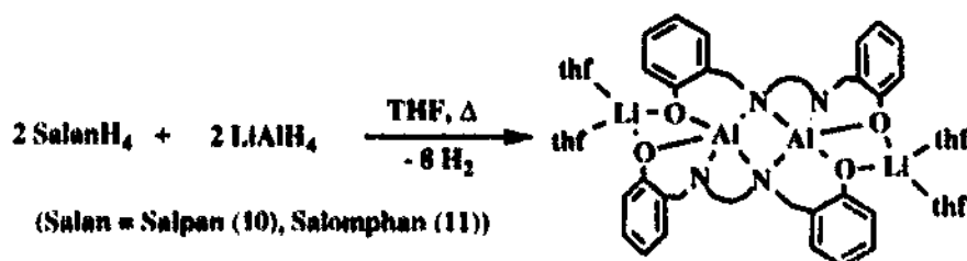
Scheme 5. The general synthesis of the dimeric Salan aluminates.
