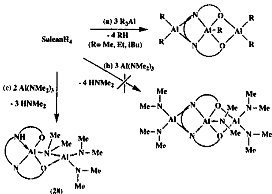
Scheme 10. The general syntheses relating to \text{SalanHAIR}(\text{Al}(\text{NMe}_2)_3) .
