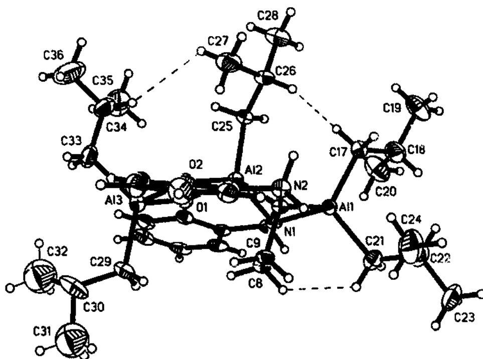
Fig. 19. Side view of the molecular structure of SalcanAl'Bu(Al'Bu 2 ) 2 (31).
