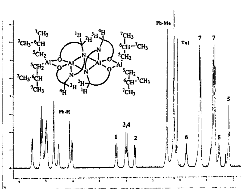
Fig. 9. ^1\text{H} NMR spectrum of [\text{SalomphanAl}(\text{Al}^i\text{Bu}_2)_2] (27).
