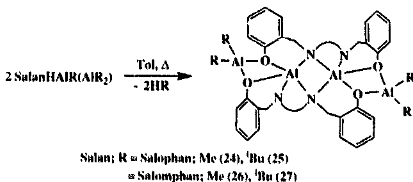
Scheme 8. General synthesis of the [\text{SalanAl}(\text{AlR}_2)]_2 derivatives.
