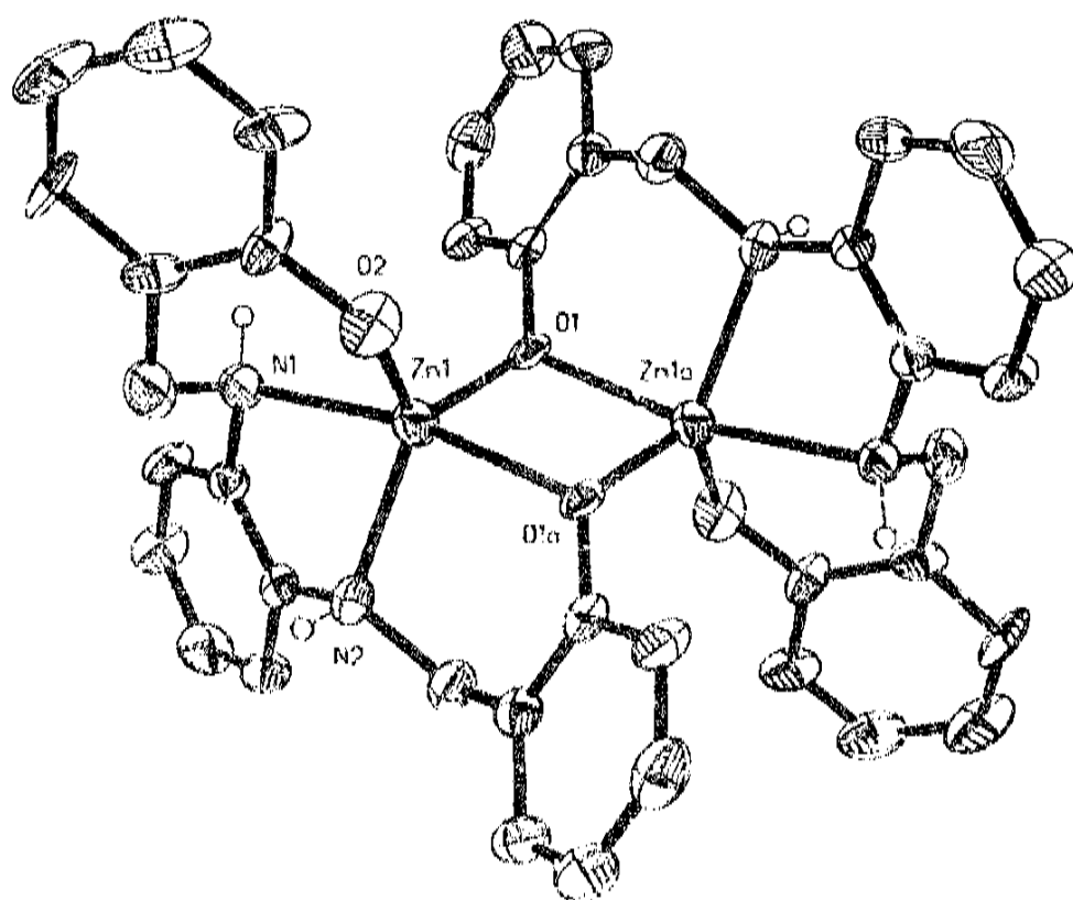
Fig. 2. Molecular structure of [SalophanH-Zn]·2SO.
