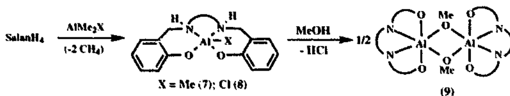
Scheme 4. Synthesis of \text{SalanH}_2\text{AlX} derivatives (with \text{X} = \text{Me}, \text{Cl} ).
