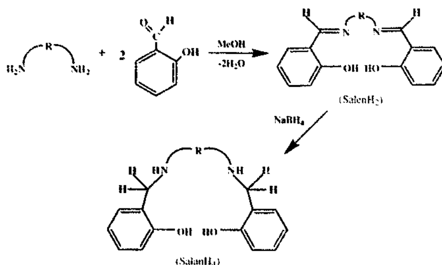
Scheme 1. General synthesis of the SalanH 2 ligands.
