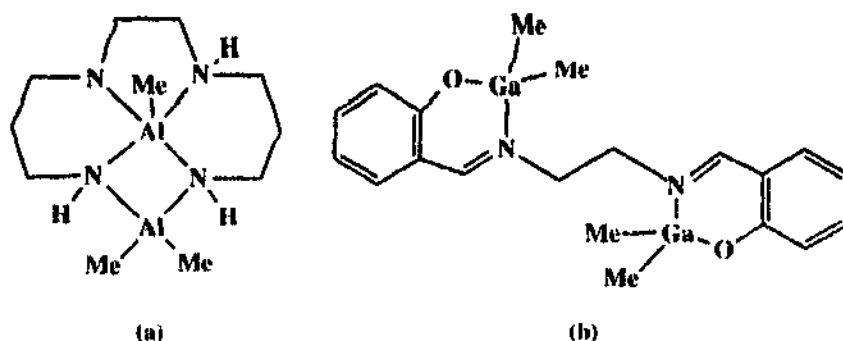
Fig. 8. Bimetallic aluminum (a) and gallium (b) complexes.
