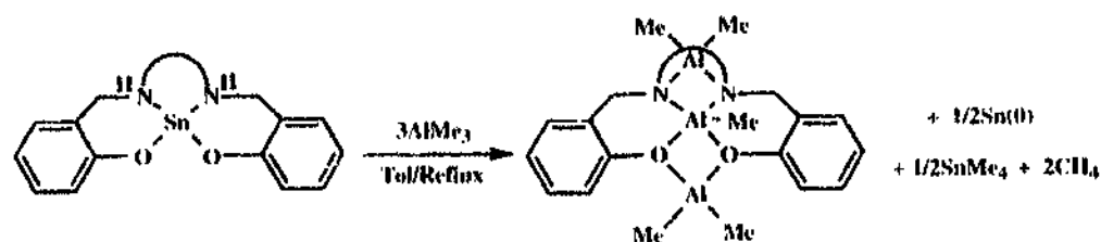
Scheme 6. Transmetalation of \text{SalanH}_2\text{Sn} to yield trimetallic aluminum derivatives.
