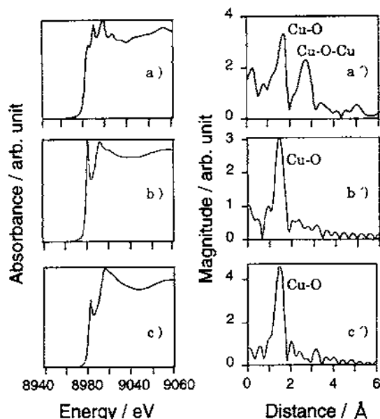
Fig. 7. XANES (a–c) and FT-EXAFS (a'–c') spectra of the \text{Cu}^+ /Y-zeolite catalysts with different Si/Al ratios: (a, a') 5.6, (b, b') 13.9, (c, c') 390.
