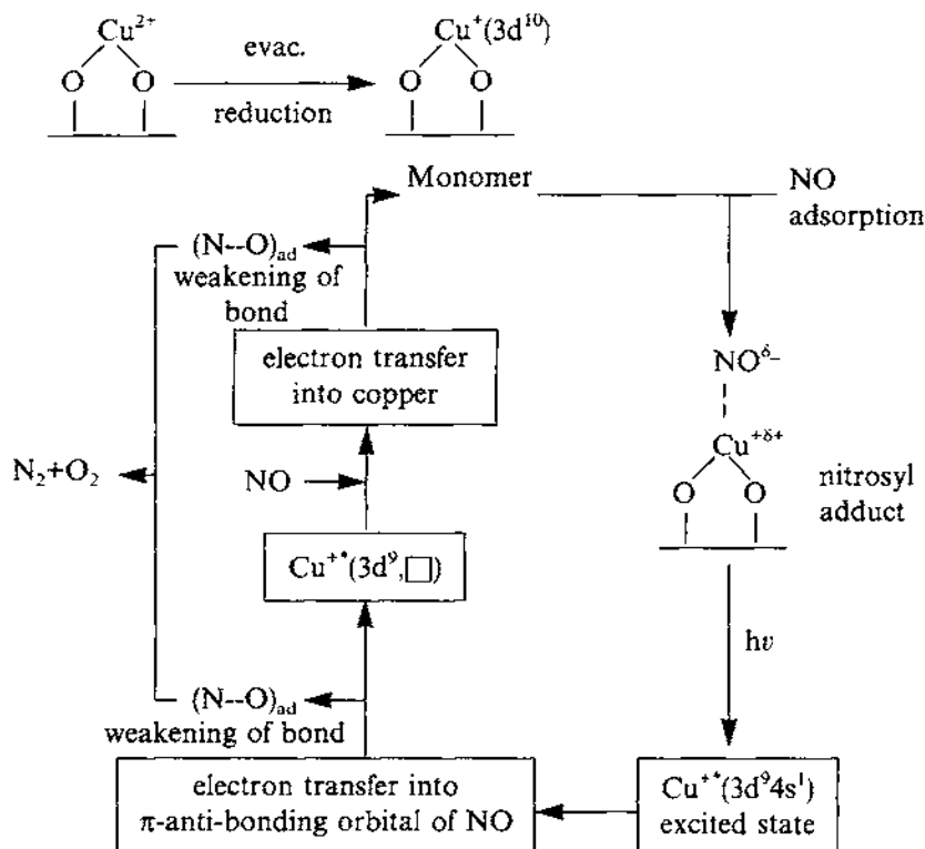
Scheme 1. Reaction scheme of the photocatalytic decomposition of NO into \text{N}_2 and \text{O}_2 on the \text{Cu}^+ /zeolite catalyst at 275 K.
