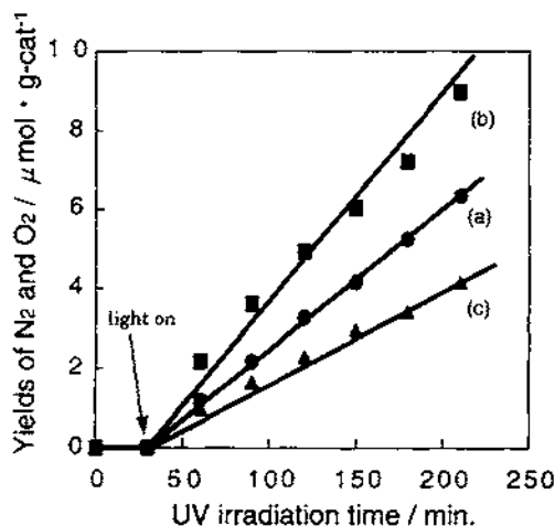
Fig. 6. Reaction profiles of the photocatalytic decomposition of \text{N}_2\text{O} into \text{N}_2 and \text{O}_2 at 275 K on the \text{Cu}^+ /Y-zeolite catalysts with different Si/Al ratios: (a) 5.6, (b) 13.9, (c) 390.
