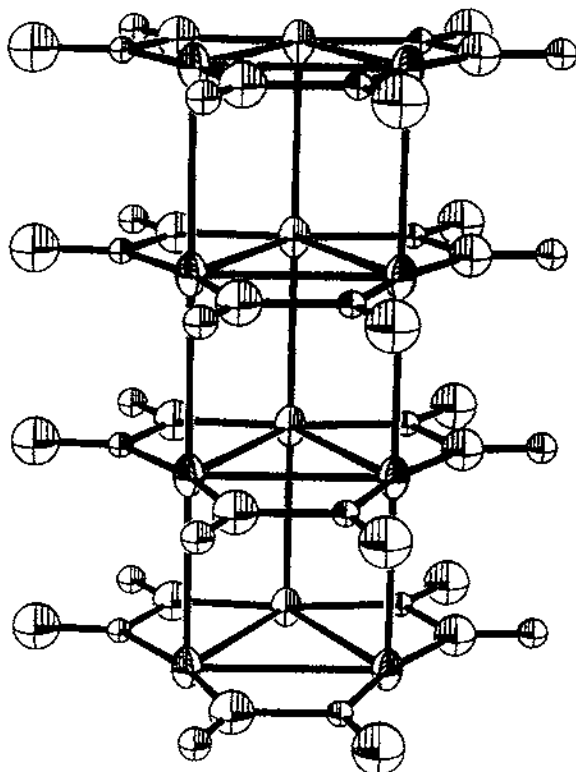
Fig. 6. A view that shows how molecules of \text{Au}_3(\text{CH}_3\text{OC}=\text{NCH}_3)_3 form a columnar structure in the solid state. The intermolecular \text{Au}\cdots\text{Au} separations are 3.346(1) \text{ \AA} , while the intramolecular \text{Au}\cdots\text{Au} separations are 3.308 \text{ \AA} (adapted from data in ref. [15]).
