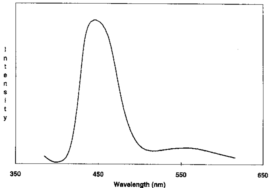
Fig. 2. The photoemission spectrum of crystalline \text{Au}_3(\text{CH}_3\text{OC}\equiv\text{NCH}_3)_3 , taken under conditions of continuous irradiation at 380 nm.
