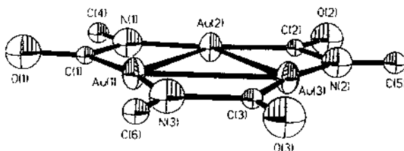
Fig. 5. The structure of an individual molecule of \text{Au}_3(\text{CH}_3\text{OC}=\text{NCH}_3)_3 (adapted from data in ref. [15]).
