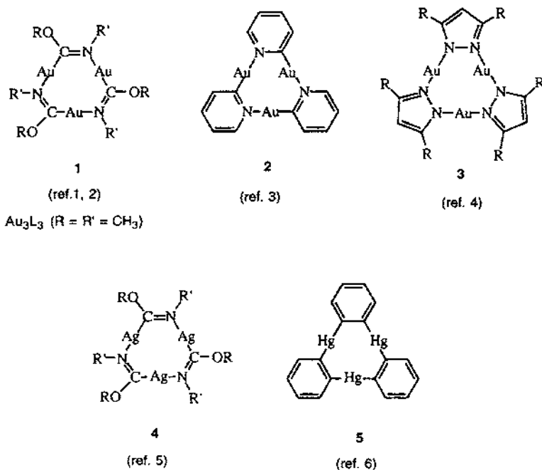
Scheme 1. Triangular metal frameworks
