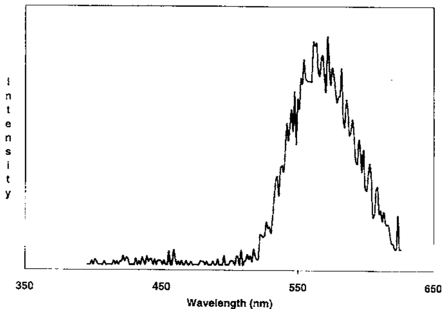
Fig. 3. Solvoluminescence: spectrum of the light emitted from a previously photo-irradiated sample of crystalline \text{Au}_3(\text{CH}_3\text{OC}\equiv\text{NCH}_3)_3 upon contact with acetone.
