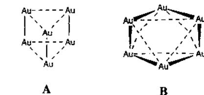
Scheme 2. Local sites within a disordered stack
