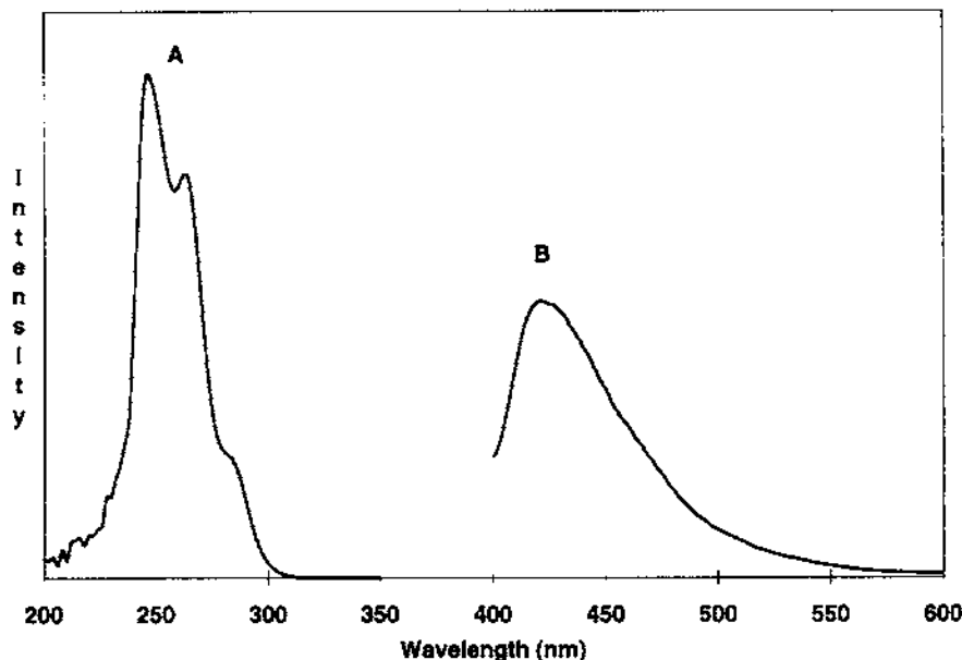
Fig. 1. The absorption (A) and emission (B) spectra of a chloroform solution of \text{Au}_3(\text{CH}_3\text{OC}=\text{NCH}_3)_3 at 25 °C. At 290 nm the extinction coefficient ( \epsilon ) is 2040 \text{ l mol}^{-1} \text{ cm}^{-1} . The excitation wavelength for the emission spectrum is 250 nm.
