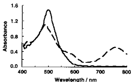
Fig. 2. Absorption spectra of the TiO 2 -supported diad 1 in the dark (dotted line) and under white light illumination (solid line). The electrode was polarized in both cases at +0.55 \text{ V/NHE} .
