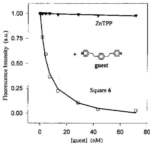
Fig. 7. Fluorescence intensity (at \lambda_{\text{em}} = 595 \text{ nm} ) of 6 (□) and ZnTPP (▽) (both at 10^{-9} \text{ M} in \text{CH}_2\text{Cl}_2 ) with addition of dipyriddy ligand guest. Solid lines correspond to the binding curve fits for ZnTPP and square 6.
