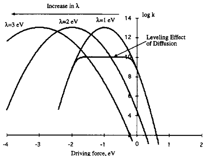
Fig. 8. The effect of higher reorganization energies ( \lambda ) on the rates of electron transfer ( k_{et} ) vs. driving force ( \Delta G^0 ) profiles predicted by the Marcus quadratic barrier relation.
