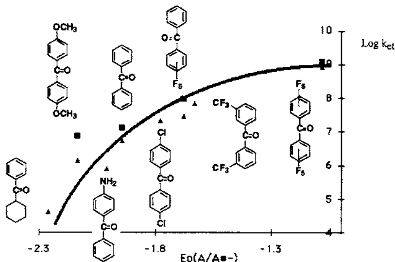
Fig. 7. \text{Log}(k_{\text{et}}) vs. E^0(\text{A}/\text{A}^{\cdot-}) for a series of benzophenone electron acceptors (A). Diamonds represent data taken in MeCN and triangles correspond to data in THF.
