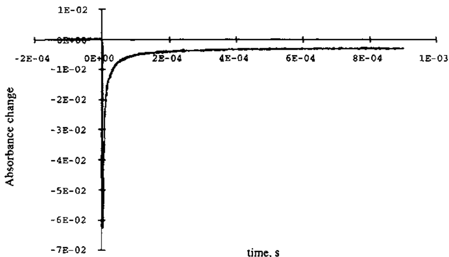
Fig. 1. Transient disappearance and reformation of the [W_2(CO)_{10}]^{2-} species in THF. \lambda_{\text{excitation}} = 355 \text{ nm} and \lambda_{\text{observation}} = 1887 \text{ cm}^{-1} .
