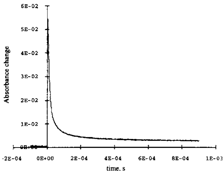
Fig. 2. Transient absorption appearance and decay of \text{W}(\text{CO})_5^- in THF: \lambda_{\text{excitation}} = 355 \text{ nm} and \lambda_{\text{observation}} = 1851 \text{ cm}^{-1} .
