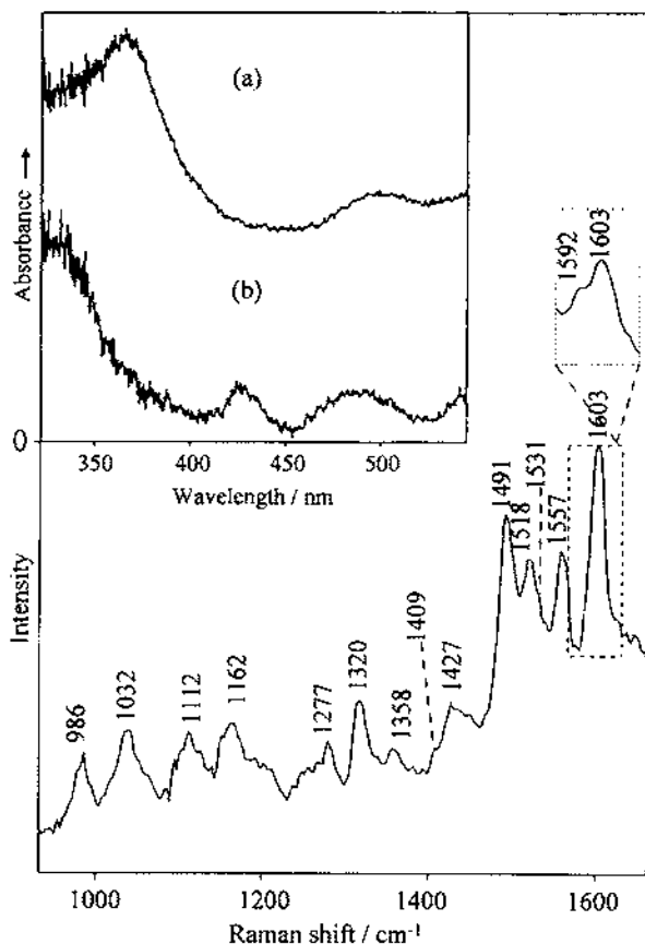
Fig. 1. Excited state RR spectra at \lambda_{ex}=355 nm using the single-colour pulse technique (laser pulse duration ca. 8 ns) of [(Ru(bpy)_2)_2bpzt]^{3+} in water; inset shows excited state absorption spectra recorded with \lambda_{ex}=416 nm of (a) [Ru(bpy)_2bpzt]^+ and (b) [(Ru(bpy)_2)_2bpzt]^{3+} , recorded using a gated multichannel diode array, 20 ns after laser excitation; the absorbance scale (arbitrary units) has been corrected for ground state depletion.
