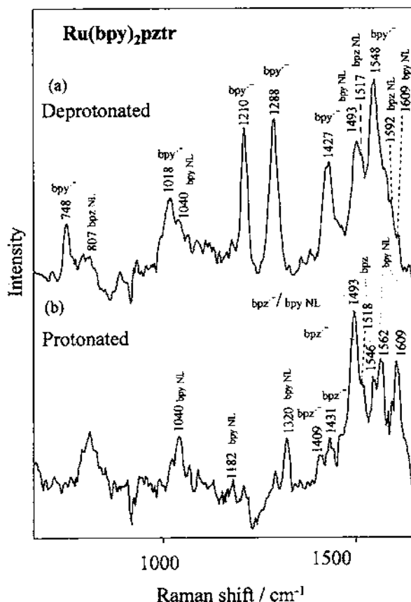
Fig. 3. Excited state RR spectra recorded at \lambda_{ex}=355 nm using the single-colour pulse technique (laser pulse duration ca. 8 ns), of [\text{Ru}(\text{bpy})_2(\text{pztr})]^+ in acetonitrile (solvent bands subtracted) with dropwise additions of: (a) diethylamine, (b) trifluoroacetic acid.
