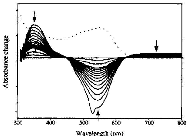
Fig. 5. Nanosecond transient absorption spectra of \text{Os}_3(\text{CO})_{10}(\text{iPr-AcPy}) in THF at 298 K. Time delay between the first 12 spectra is 10 ns, after that it is 30 ns (--- = ground state absorption).
