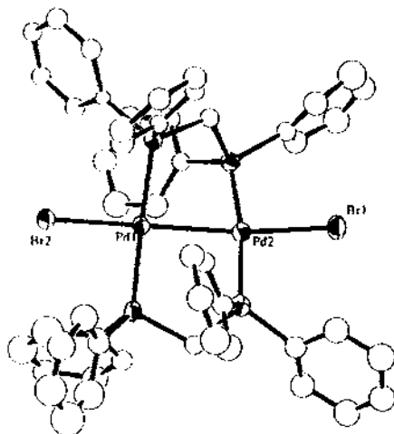
Fig. 2. The molecular structure of [\text{Pd}_2\text{Br}_2(\text{dppm})_2] .
