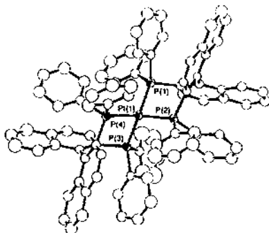
Fig. 4. An ORTEP drawing of [\text{Pt}((S)\text{-BINAP})_2] .
