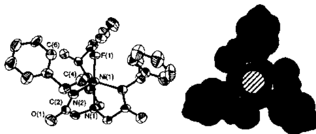
Fig. 5. Thermal ellipsoid diagram of [\text{NiI}^{\text{S-mbz}}(\text{F})]^{2-} and a space-filling representation of the complex. The ellipsoids are drawn at the 40% probability level and hydrogens are omitted for clarity. Selected bond distances (Å) and angles ( ^{\circ} ): \text{Ni}(1)-\text{F}(1)=1.950(6) ; \text{Ni}(1)-\text{N}(1)=2.104(10) ; \text{Ni}(1)-\text{N}(2)=2.073(4) ; \text{C}(6)-\text{F}(1)=3.165 ; \text{N}(1)-\text{Ni}(1)-\text{F}(1)=180.000(2) ; \text{N}(2)-\text{Ni}(1)-\text{F}(1)=100.86(11) ; \text{N}(2)-\text{Ni}(1)-\text{N}(1)=79.15(11) ; \text{N}(2)-\text{Ni}(1)-\text{N}(2)\#2=116.54 .
