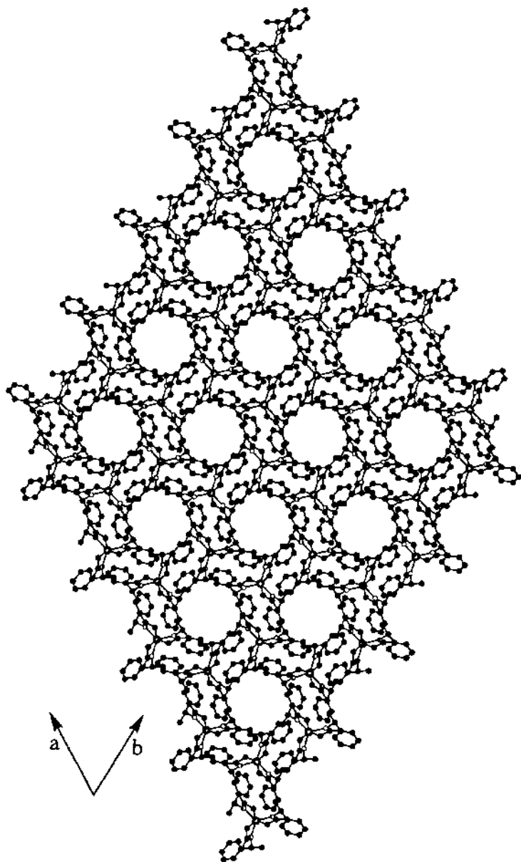
Fig. 8. A portion of the crystal lattice for [\text{Ni}(\text{S-mba})(\text{F})]^{2-} (viewed along the a, b plane). The \text{Et}_4\text{N}^+ ions and the hydrogens have been omitted for clarity.
