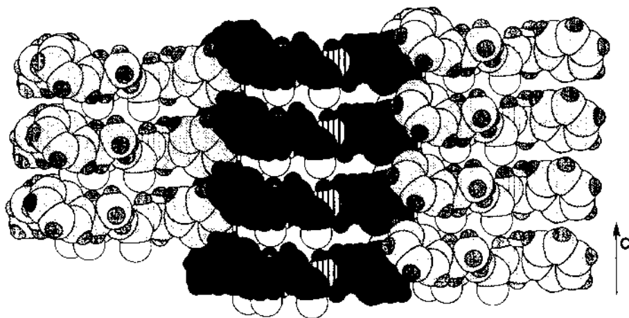
Fig. 4. The crystal structure of H_3I^{S-mbz} showing the intercolumn interactions within the crystal lattice (view of the b, c plane).
