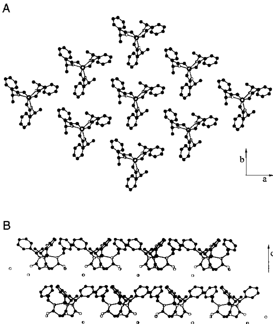
Fig. 6. A portion of the crystal lattice for [\text{Ni}1^{\text{S-mbz}}(\text{F})]^{2-} \cdot \text{Et}_4\text{N}^+ (A) (viewed along the a, b plane) and (B) (viewed along the b, c plane) showing the positions of the nitrogen atoms of the \text{Et}_4\text{N}^+ ions. Hydrogens have been omitted for clarity.
