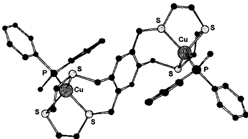
Fig. 1. The X-ray structure of the cation anti -[Cu 2 L(PPh 2 Me) 2 ] 3+ [L=(17)] [18].
