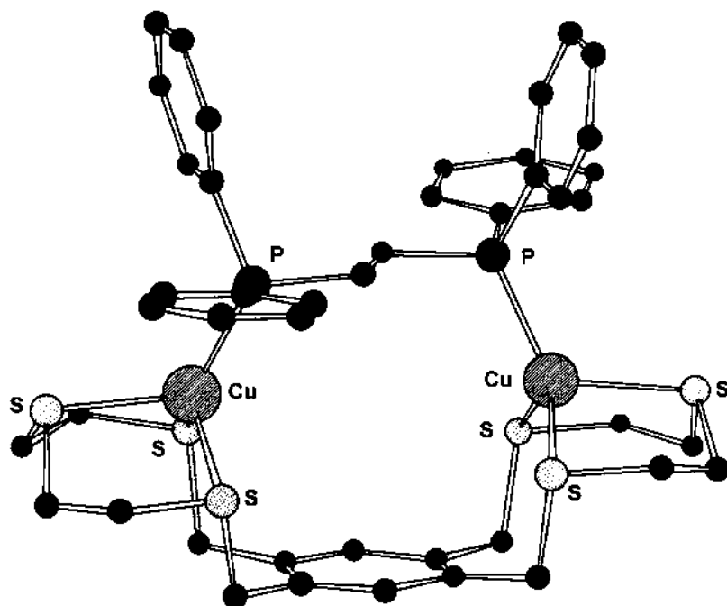
Fig. 2. The X-ray structure of the cation \text{syn}[\text{Cu}_2\text{L}(\mu\text{-PPh}_2\text{CH}_2\text{CH}_2\text{PPh}_2)]^{2+} [ \text{L}=(17) ] [28].
