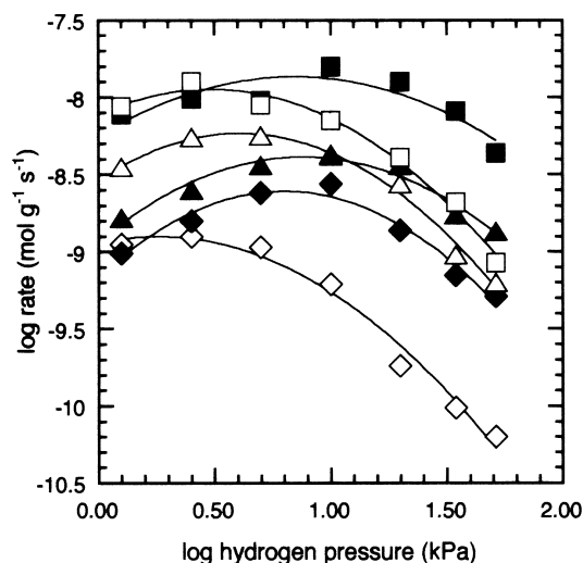
Fig. 3. Hydrogen pressure dependence for the rate of \alpha\gamma (full symbols) and \alpha\delta (open symbols) routes in TeMB hydrogeolysis at 463 K on small metallic particles of Ru/Al 2 O 3 (□, ■), RuSn/Al 2 O 3 (▲, △) and RuGe/Al 2 O 3 (◇, ◆).
