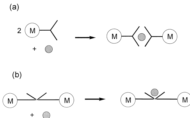
Fig. 3. Schematic representation of how complexation of a metal cation (shaded sphere) can promote (a) extension of the molecular axis and (b) perturbation of the energetics of the bridge.
