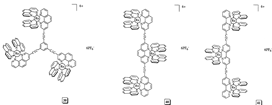
Fig. 34. Structures of the various trinuclear Ru(II) complexes.
