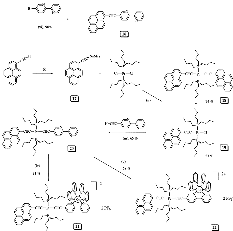
Fig. 16. Synthetic route used to attach one ( 19 , 20 ) or two ( 18 ) pyrene units to a central \text{Pt}^{\text{II}} bis-acetylide. The mono-derivative ( 19 ) is the key intermediate for further functionalization to give the Ru–Pt–pyrene ( 22 ) and Os–Pt–pyrene ( 21 ) photoactive dyads. These latter compounds require isolation of the important building block 20 that contains a vacant 2,2'-bipyridine ligand: (i) (a) n\text{-BuLi} , THF, -78^\circ\text{C} , 2 h, (b) \text{SnMe}_3\text{Cl} ; (ii) \text{CuI} (1 mol%), THF, 60^\circ\text{C} , 2 days; (iii) \text{CuI} (1 mol%), (^i\text{Pr})_2\text{NH} , THF, 25^\circ\text{C} , 5 days; (iv) 1 equiv. [\text{Os}(\text{bpy})_2\text{Cl}_2] , \text{C}_2\text{H}_5\text{OH} , 80^\circ\text{C} , 1 day; (v) 1 equiv. [\text{Ru}(\text{bpy})_2\text{Cl}_2] \cdot 2\text{H}_2\text{O} , \text{C}_2\text{H}_5\text{OH} , 80^\circ\text{C} , 1 day; (vi) [\text{Pd}^0(\text{PPh}_3)_4] 6 mol%, \text{C}_6\text{H}_6 , (^i\text{Pr})_2\text{NH} , 80^\circ\text{C} , 15 h.
