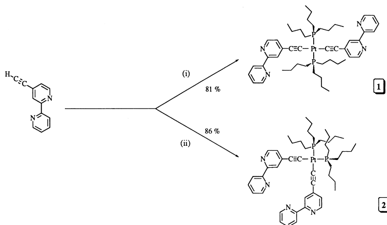
Fig. 6. Synthesis of “linear” ( 1 ) and “bent” ( 2 ) \text{Pt}^{\text{II}} bis- \sigma -acetylides bearing vacant 2,2'-bipyridyl ligands suitable for subsequent complexation of incoming metallo-fragments: (i) \text{trans-[Pt}^{\text{II}}(\text{nBu}_3\text{P})_2\text{Cl}_2] , \text{CuI} (ca. 1 mol%), (\text{iPr})_2\text{NH} , THF, 25 °C, 5 days; (ii) \text{cis-[Pt}^{\text{II}}(\text{nBu}_3\text{P})_2\text{Cl}_2] , \text{CuI} (ca. 1 mol%), (\text{iPr})_2\text{NH} , THF, 25 °C, 5 days.
