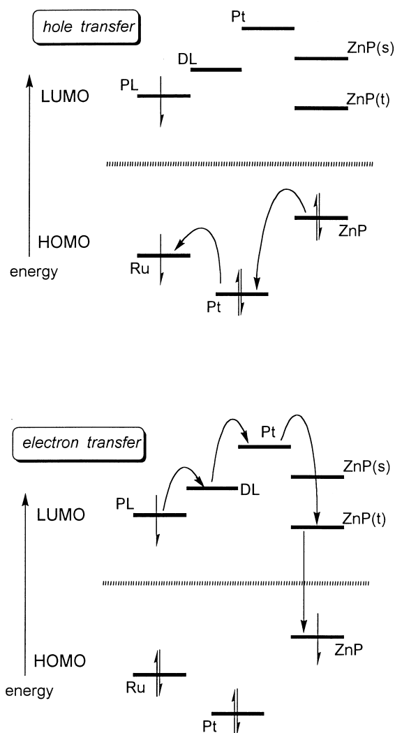
Fig. 20. Projected pathways for forward and reverse electron transfer in the ZnP-Pt II -Ru II tripartite complex ( 15 ) following selective excitation into the terminal Ru II complex. Forward reaction is expected to proceed via hole transfer involving the respective HOMOs and forming Pt III as a virtual intermediate. Charge recombination is expected to proceed by way of a cascade of electron-transfer steps involving the various LUMOs. This latter process results in partial population of the triplet excited state of ZnP.
