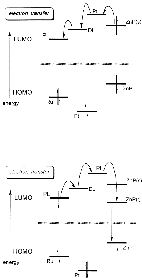
Fig. 19. Projected pathways for forward and reverse electron transfer in the ZnP–Pt II –Ru II tripartite complex ( 15 ) following selective excitation into ZnP. Both reactions are expected to occur via a cascade of electron-transfer steps involving intermediary (or virtual) reduction of Pt II , the ditopic ligand (DL), and the parent ligand (PL). The two reactions take place through the LUMOs and, therefore, are designated as electron-transfer processes.
