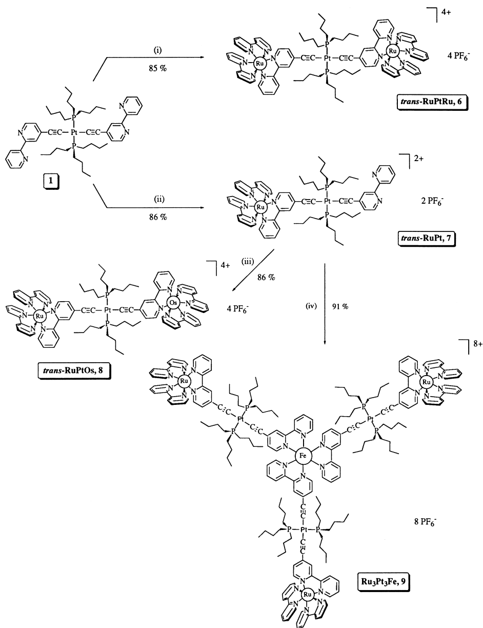
Fig. 8. Synthetic route used to prepare heteropolynuclear complexes using Pt II σ-acetylides as spacers: (i) 2 equiv. [Ru(bpy) 2 Cl 2 ]·2H 2 O, C 2 H 5 OH, 80 °C, 15 h; (ii) 1 equiv. [Ru(bpy) 2 Cl 2 ]·2H 2 O, C 2 H 5 OH, 80 °C, 15 h; (iii) 1 equiv. [Os(bpy) 2 Cl 2 ], C 2 H 5 OH, 90 °C, 3 days; (iv) ca. 0.4 equiv. FeSO 4 ·7H 2 O, C 2 H 5 OH/H 2 O, 25 °C, 10 min exposure to ultrasonic irradiation.
