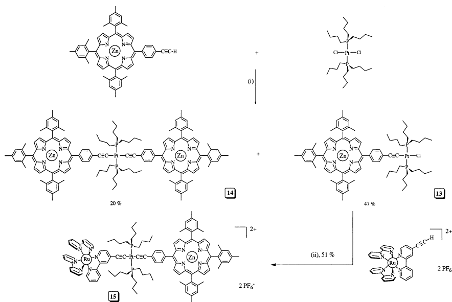
Fig. 14. Synthetic route used to prepare the mono- ( 13 ) and binuclear ( 14 ) ZnP derivatives containing a \text{Pt}^{\text{II}} \sigma -acetylide function as substituent or bridge. The mononuclear complex 13 is used in subsequent reactions to prepare the ZnP– \text{Pt}^{\text{II}} – \text{Ru}^{\text{II}} tripartite complex 15 : (i) \text{CuI} (1 mol%), (^i\text{Pr})_2\text{NH} , THF, 25 °C, 7 days; (ii) \text{CuI} (1 mol%), (^i\text{Pr})_2\text{NH} , \text{CH}_3\text{CN}/\text{THF} , 25 °C, 3 days.
