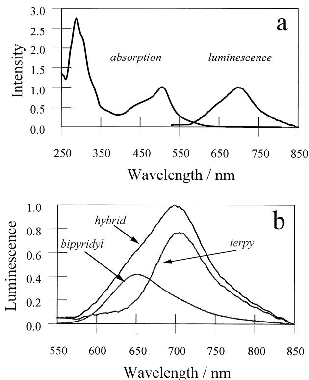
Fig. 31. (a) Absorption and emission spectra recorded for the binuclear Ru II hybrid complex 34 in deoxygenated acetonitrile at 20 °C. (b) Deconstruction of the emission spectrum into components associated with the bipyridyl- and terpyridyl-based mononuclear complexes. This deconstruction procedure gives a good representation of the spectrum recorded for the hybrid complex.
