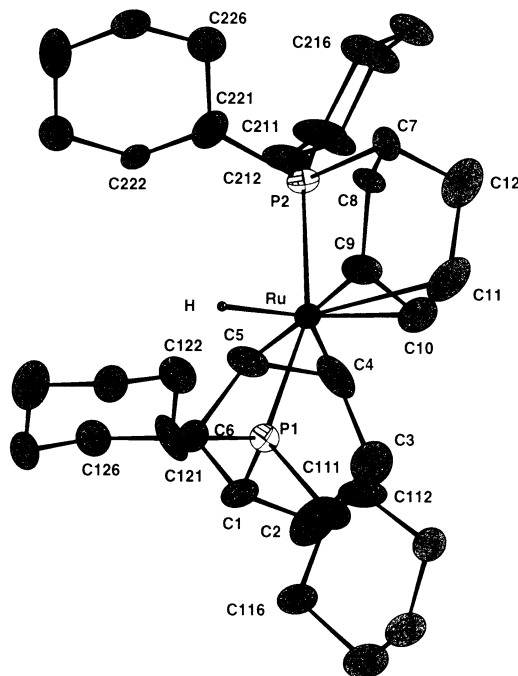
Fig. 7. The structure of 54 , showing the (\eta^3\text{-C}_6\text{H}_8)\text{PCy}_2 and the (\eta^2\text{-C}_6\text{H}_9)\text{PCy}_2 ligands.
