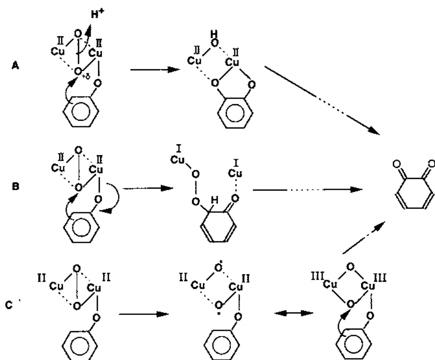
Fig. 8. Possible mechanistic pathways for step (i) (see Fig. 7).
