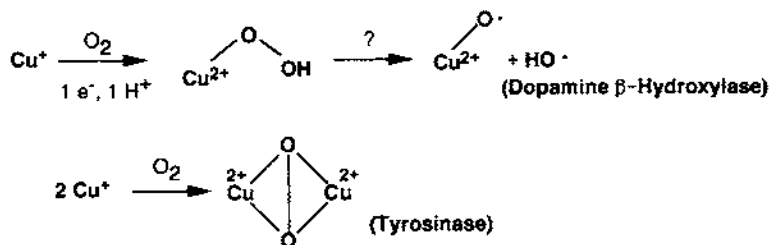
Fig. 3. Intermediate in dopamine \beta -hydroxylase and tyrosinase.
