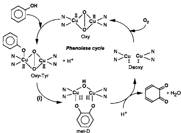
Fig. 7. Proposed mechanism for phenolase activity of tyrosinase (adapted from [8]).
