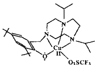
Fig. 12. Tolman model for GOase (from Ref. [19]).
