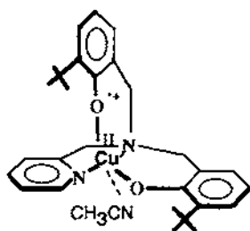
Fig. 11. A model for the active form of GOase (from Ref. [18]).
