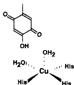
Fig. 13. The active site in PSAO.
