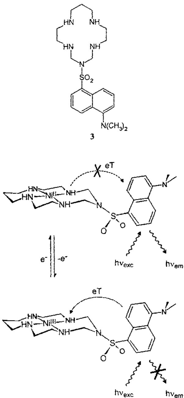
Fig. 7. Sketch of the fluorescence switching activity of the [Ni^{III}](3)]^{3+ \cdot 2+} system. The Ni^{III} centre promotes a fluorophore-to-metal electron transfer and quenches dansyl fluorescence. The Ni^{II} -to-dansyl electron transfer process is thermodynamically disfavoured. Thus, the Ni^{III} -to- Ni^{II} reduction restores fluorescence.
