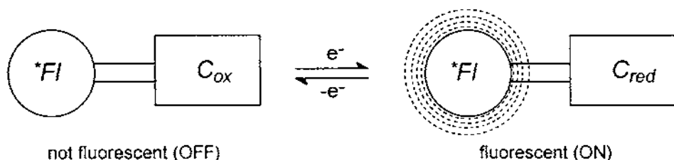
Fig. 1. The multicomponent approach to the design of a redox switch of fluorescence. Switch efficiency requires that the control unit C in its oxidized form, C_{ox} , quenches the proximate photo-excited fluorophore FI^* and the reduced form C_{red} does not (OFF/ON switch). The other favourable ON/OFF situation can be obtained when C_{red} quenches FI^* and C_{ox} does not.
