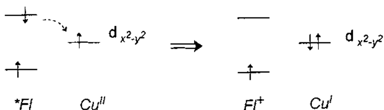
Fig. 5. Details of an electron transfer process (double-electron exchange mechanism) involving an excited fluorophore and a d^9 metal ion in an octahedrally elongated coordinative arrangement.
