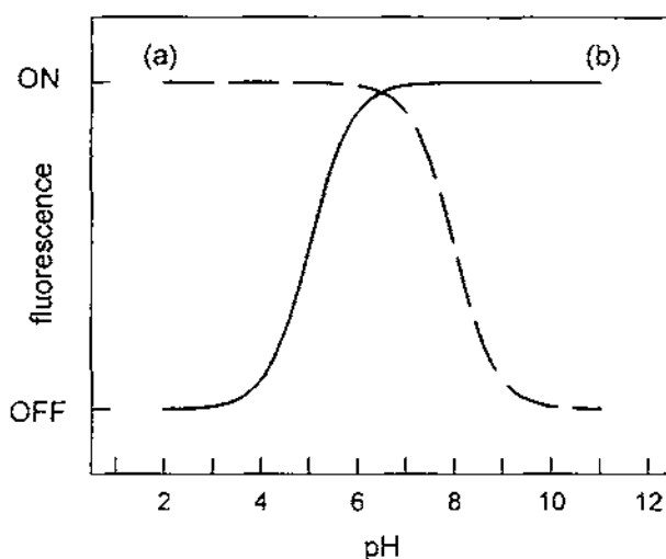
Fig. 8. Calculated fluorescence versus pH sigmoidal profiles for multicomponent system (acid/base fragment-spacer-fluorophore) of type 8 (a: ON/OFF response, pK_A = 5 ) and of type 9 (b: OFF/ON response, pK_A = 8 ).
