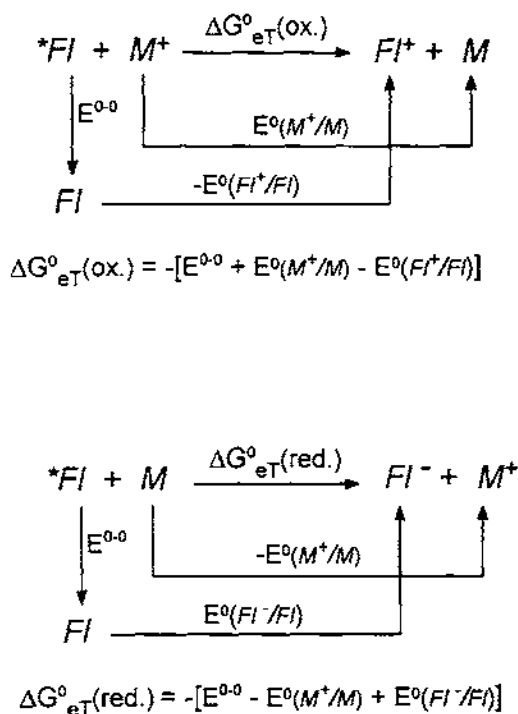
Fig. 6. Thermodynamic aspects of photo-induced electron transfer processes involving a fluorophore FI and a metal centred redox couple M^+/M .
