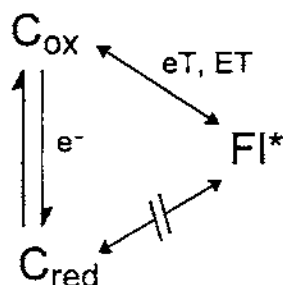
Fig. 2. The basis of an OFF/ON redox switch of fluorescence. Either an energy transfer (ET) or an electron transfer (eT) mechanism can be responsible for the quenching of the light emitting fragment FI^* , in a multicomponent redox unit-spacer-fluorophore system C \sim FI .
