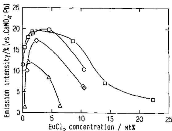
Fig. 13. The dependence of emission intensity of \text{Eu}^{2+} -copoly(MA15C5/X) (1:5) complex on \text{EuCl}_2 concentration: (a) X=\text{MMA} ( \circ ); (b) X=\text{EMA} ( \square ); (c) X=\text{BMA} ( \triangle ); (d) X=\text{MAG1} ( \diamond ).
