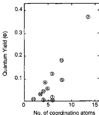
Fig. 7. The relationship between quantum yield and coordination numbers of \text{Eu}^{2+} in complexes in methanol with the ligand of: 2, 15C5; 3, 18C6; 4, dicyclohexyl-18-crown-6 (DC18C6); 5, dicyclohexyl-24-crown-8 (DC24C8); 6, B15C5; 7, B18C6; 9, cryptand [2.2]; 11, cryptand [2.2.1]; 12, cryptand [2.2.2]; 15, pentaethylene glycol (EO5); 16, hexaethylene glycol (EO6); 17, heptaethylene glycol (EO7).
