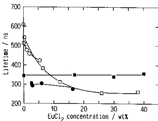
Fig. 14. The dependence of luminescence lifetime of \text{Eu}^{2+} polymer or copolymer complex on \text{EuCl}_2 concentration: (a) \text{Eu}^{2+} -PMA15C5 (□); (b) \text{Eu}^{2+} -copoly(MA15C5/MMA) (1:10) (○); (c) \text{Eu}^{2+} -PMA18C6 (■); (d) \text{Eu}^{2+} -copoly(MA18C6/MMA) (1:10) (●).
