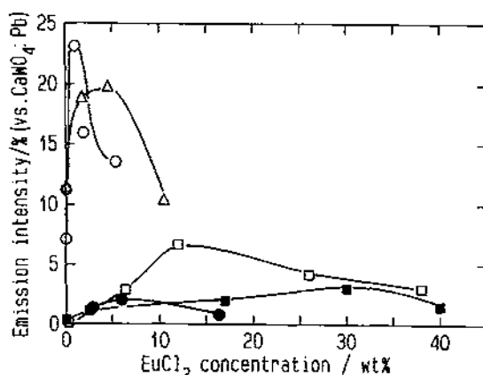
Fig. 11. The dependence of emission intensity of \text{Eu}^{2+} polymer or copolymer complex on \text{EuCl}_2 concentration: (a) \text{Eu}^{2+} -PMA15C5 (Δ); (b) \text{Eu}^{2+} copoly(MA15C5/MMA) (1:5) (Δ); (c) \text{Eu}^{2+} -copoly(MA15C5/MMA) (1:10) (○); (d) \text{Eu}^{2+} -PMA18C6 (■); (e) \text{Eu}^{2+} -copoly(MA18C6/MMA) (1:10) (●).
