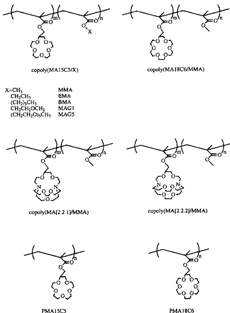
Scheme 2. The schematic structure of crown ether- or cryptand-containing polymer or copolymer ligands.
