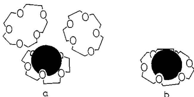
Fig. 4. Structural configuration of \text{Eu}^{2+} complex in alcohol solution: (a) \text{Eu}^{2+} –15C5; (b) \text{Eu}^{2+} –18C6.
