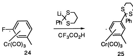
Scheme 8. Tele-meta S_NAr
