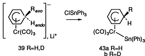
Scheme 15. Formation of a dinuclear \text{Cr}-\text{Sn}(\eta^5\text{-cyclohexadienyl}) complex
