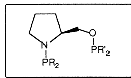
R, R' = Me, iPr, Cp, Cy, Ph, Nm (α-naphthyl)methyl Ph,Cy-ProNOP Cy,Ph-ProNOP ProNOP* Ph,iPr-ProNOP Me-ProNOP iPr,Ph-ProNOP iPr-ProNOP Ph,Cp-ProNOP Cp-ProNOP Cp,Ph-ProNOP Cy-ProNOP iPr,Cp-ProNOP Nm-ProNOP Cp,iPr-ProNOP Cy,Cp-ProNOP Cp,Cy-ProNOP
