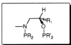
R = R' = Ph, R 1 = Ph isoPheGlyNOP Cp,Cp-isoAlaNOP Cy,Cy-isoAlaNOP R, R' = Cp, Cy, Ph } R 1 = Me } Cy,Cp-isoAlaNOP Cp,Cy-isoAlaNOP Ph,Cp-isoAlaNOP
