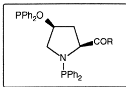
R = OEt E-ProNOP R = O(CH 2 ) 2 OEt E,E-ProNOP R = NHBu Bu-ProNOP R = OEt, and P(iPr) 2 iPr-E-ProNOP
