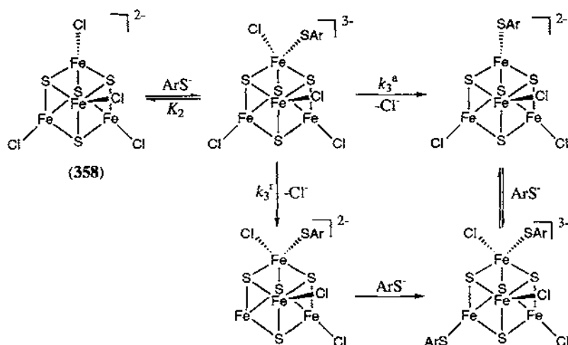
Scheme 8.
