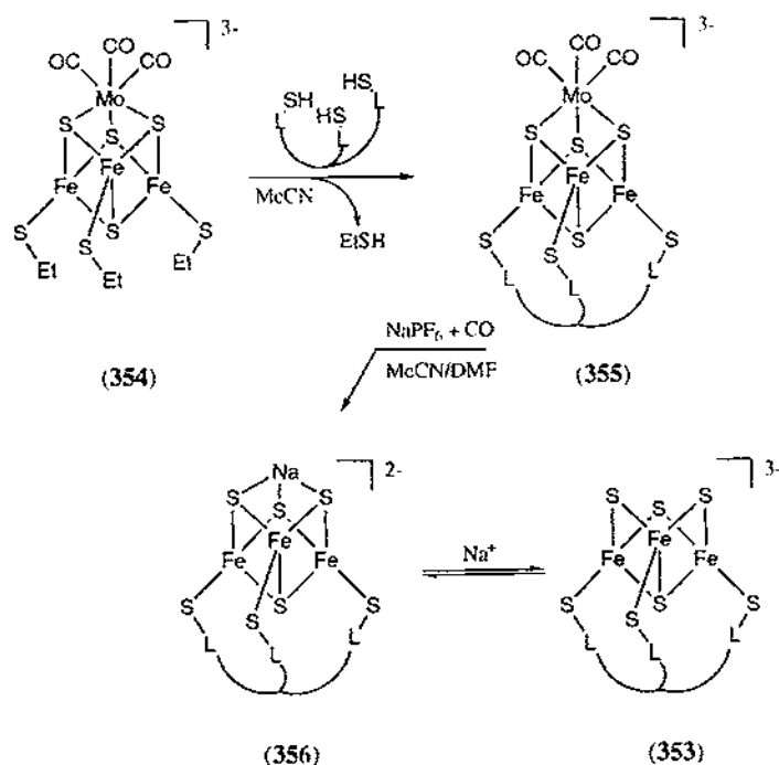
Scheme 7.
