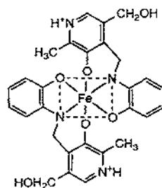
(240) estimated structure
