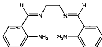
\text{H}_2(\mathbf{59})
