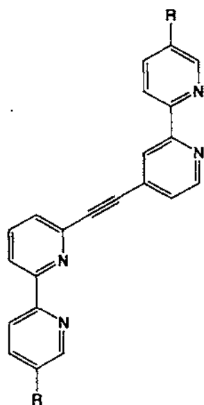
(22; R=H, Me)
