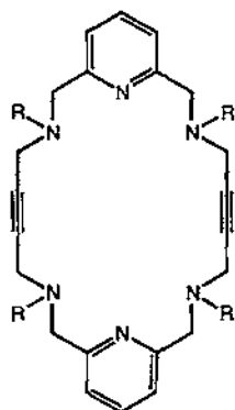
(148) R=C_{16}H_{33}
