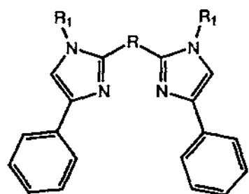
(116), \text{R}_1 = \text{Et}
