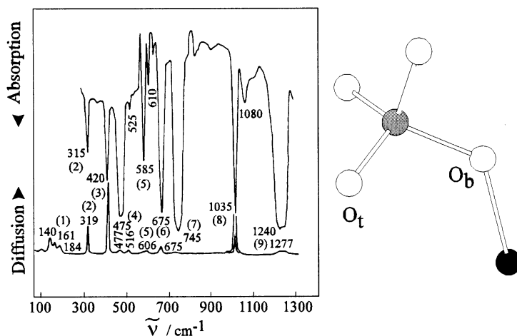
Fig. 13. IR and Raman spectra of \text{GeCl}_3\text{ClO}_4 . (1) lattice vibrations + def. \text{GeCl}_3 + \delta\text{GeOCl} , (2) \rho_r\text{ClO}_3 , (3) \nu_s\text{GeCl}_3 , (4) \nu_{as}\text{GeCl}_3 + \delta_s\text{ClO}_4 , (5) \delta_{as}\text{ClO}_4 , (6) \nu\text{GeO}(\text{ClO}_4) , (7) \nu\text{ClO}_b , (8) \nu_s\text{ClO}_t , (9) \nu_{as}\text{ClO}_t . def: deformation including \delta and \rho ; \text{O}_b : bridging oxygen; \text{O}_t : non bonded Cl–O.
