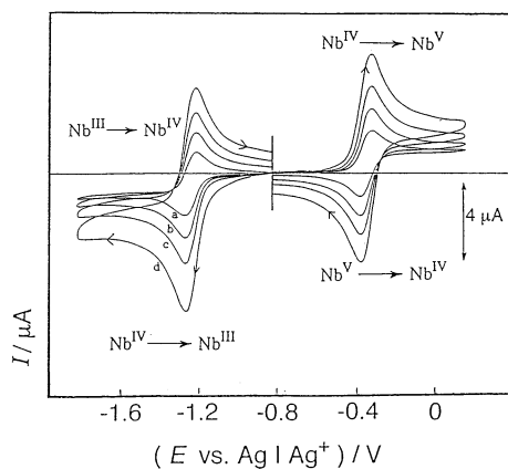
Fig. 4. Cyclic voltammetry of \text{Cp}_2\text{Nb}(\text{dmit}) [70].
