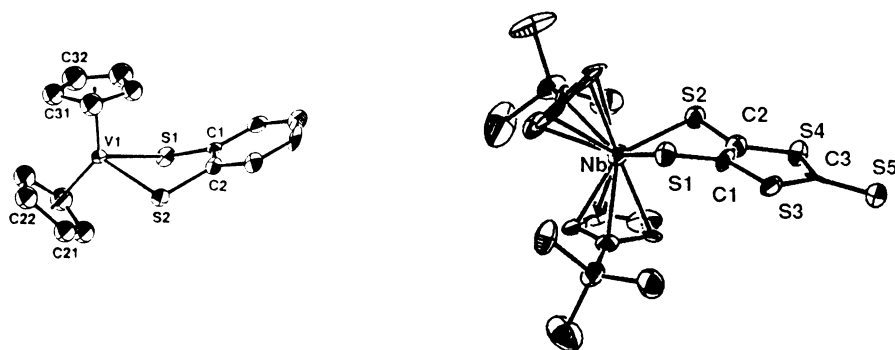
Fig. 5. ORTEP views of \text{Cp}_2\text{V}(\text{bdt}) (left) [23] and (\text{Me}_3\text{SiCp})_2\text{Nb}(\text{dmit}) (right) [9].
