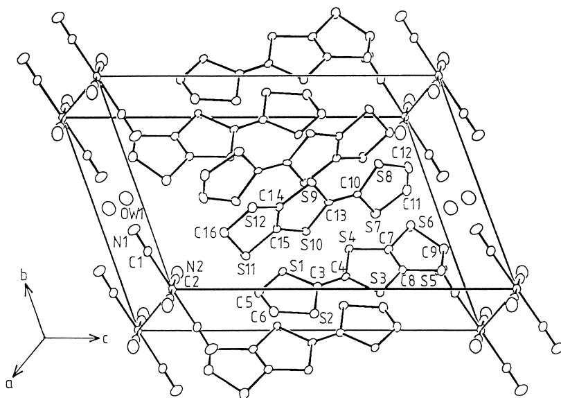
Fig. 12. Crystal structure of \kappa -(MDT-TTF) 4 [M(CN) 6 ].(CH 2 Cl 2 ) 2 .
