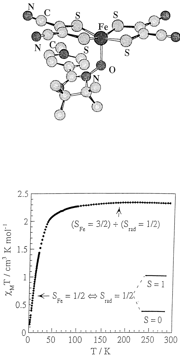
Fig. 17. Molecular structure and temperature dependence of the \chi_M T product for \text{Fe}(\text{mnt})_2\text{-rad} .
