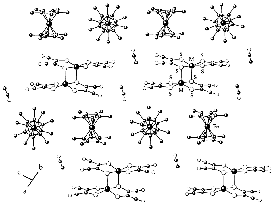
Fig. 16. Crystal structure of \alpha\text{-[Fe(Cp}^*)_2]_2[\text{M(mnt)}_2]_2 , \text{M} = \text{Fe(III)} and \text{Co(III)} .
