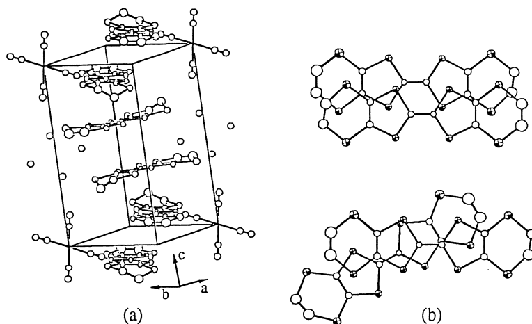
Fig. 9. Crystal structure of \delta\text{-(ET)}_4[\text{Ni(CN)}_4]_x[\text{Pt(CN)}_4]_{1-x}\cdot(\text{H}_2\text{O})_n .
