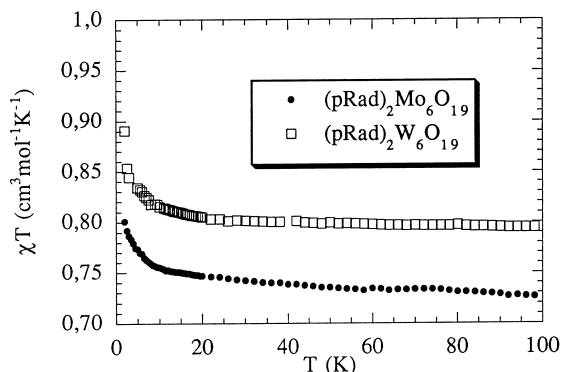
Fig. 2. \chi_M T vs. T curve in the 2–100 K temperature range for (p\text{-rad})_2[M_6O_{19}] .
