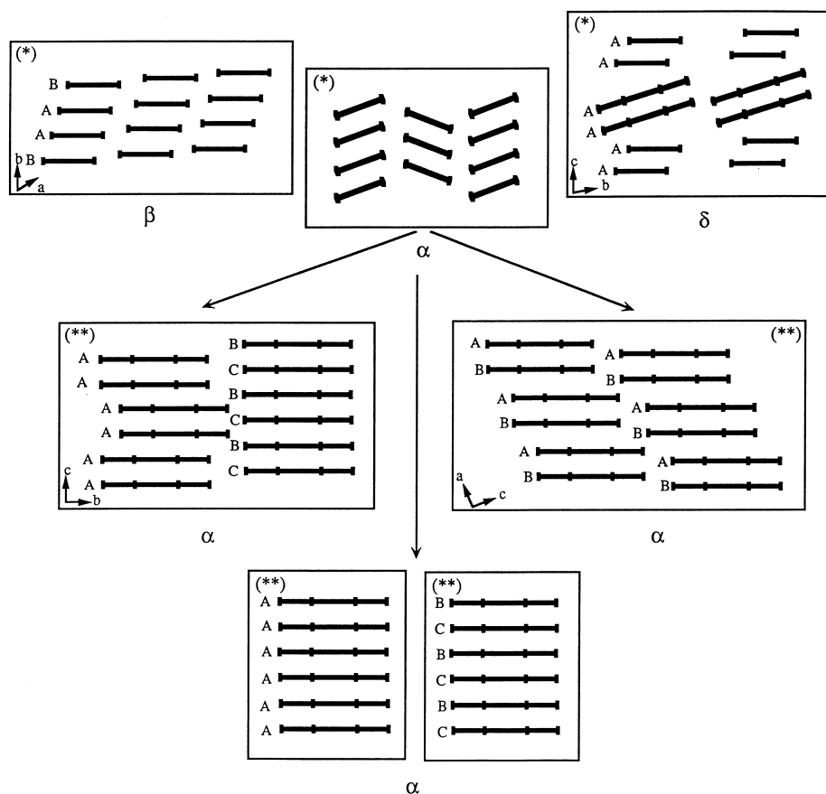
Fig. 11. Schematic diagrams of the different structural types \alpha_1 , \alpha_2 , \beta and \delta encountered in the ET/M(CN) 4 systems compared with \alpha -(ET) 2 MHg(SCN) 4 ·( \alpha 0) [117]. Views along the main (*) and minor (**) molecular axes of the ET unit are represented.
