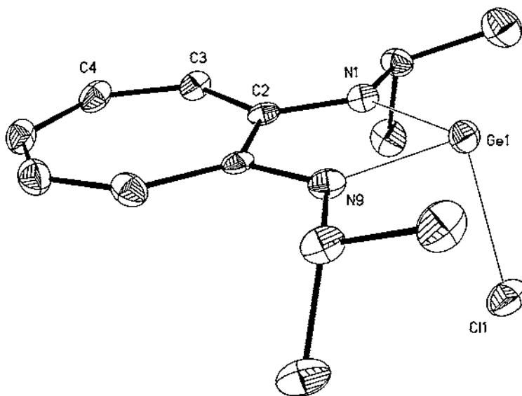
Fig. 9. Molecular structure of \{[(i\text{-Pr})_2\text{ATI}]\text{GeCl}\} . Reprinted with permission from Dias et al. [30] © 1997 American Chemical Society. Selected bond lengths (Å) and angles (°): Ge1–N1, 1.956(4); Ge1–N9, 1.956(4); Ge1–Cl1, 2.364(2); N1–C2, 1.338(6); N9–C8, 1.341(6); N1–Ge–N9, 80.2(2); Cl1–Ge–N1, 97.13(13); Cl1–Ge–N9, 96.87(13).
