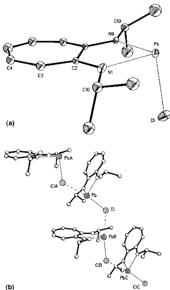
Fig. 11. Molecular structure of [(i\text{-Pr})_2\text{ATI}]\text{PbCl} . A. ORTEP diagram. B. A view showing intermolecular interactions. Selected bond lengths (Å) and angles (°): \text{Pb–N1} , 2.265(13); \text{Pb–N9} , 2.249(13); \text{Pb–Cl} , 2.780(4); \text{Pb} \cdots \text{Cl} , 3.095; \text{N1–C2} , 1.32(2); \text{N9–C8} , 1.33(2); \text{N1–Pb–N9} , 70.3(4); \text{Cl–Pb–N1} , 91.3(3); \text{Cl–Pb–N9} , 95.5(3); \text{Cl–Pb} \cdots \text{Cl} , 170.3.
