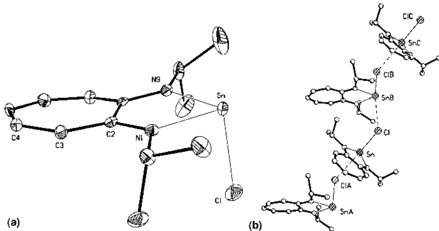
Fig. 10. Molecular structure of \{[(i\text{-Pr})_2\text{ATI}]\text{SnCl}\} . A. ORTEP diagram. B. A view showing intermolecular interactions. Reprinted with permission from Dias et al. [29] © 1996 American Chemical Society. Selected bond lengths (Å) and angles (°): Sn–N1, 2.164(5); Sn–N9, 2.164(5); Sn–Cl, 2.542(2); Sn...ClA, 3.558; N1–C2, 1.332(7); N9–C8, 1.331(7); N1–Sn–N9, 73.9(2); Cl–Sn–N1, 92.44(13); Cl–Sn–N9, 94.13(12); Cl–Sn...ClA, 172.3.
