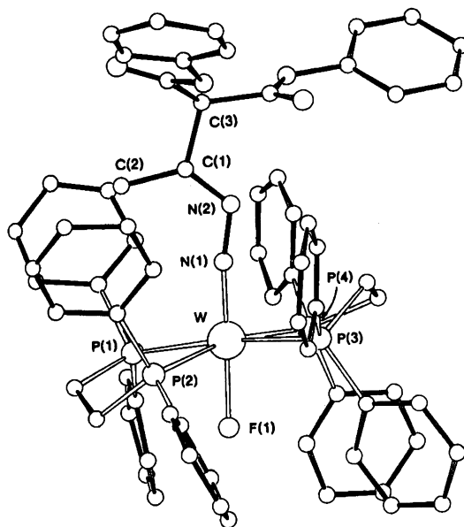
Fig. 3. ORTEP drawing of trans[WF(NN= CMeCH (CONHPh) _2 )(dpe) _2 ][BF _4 ] ( 10c ) from Refs. [17,18].
