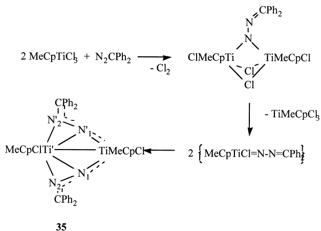
Scheme 18. Reaction of \text{N}_2\text{CPh}_2 on \text{MeCpTiCl}_3
