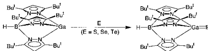
Scheme 3.
