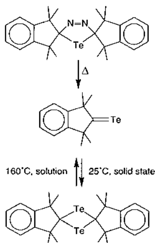
Scheme 5.
