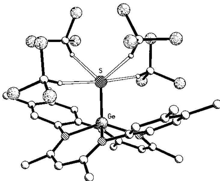
Fig. 11. E...H–CCl 3 hydrogen-bonding interactions in [\eta^4\text{-Me}_8\text{taa}]ME (M = Ge, Sn; E = S, Se).
