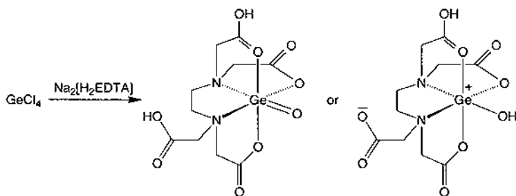
Scheme 15.
