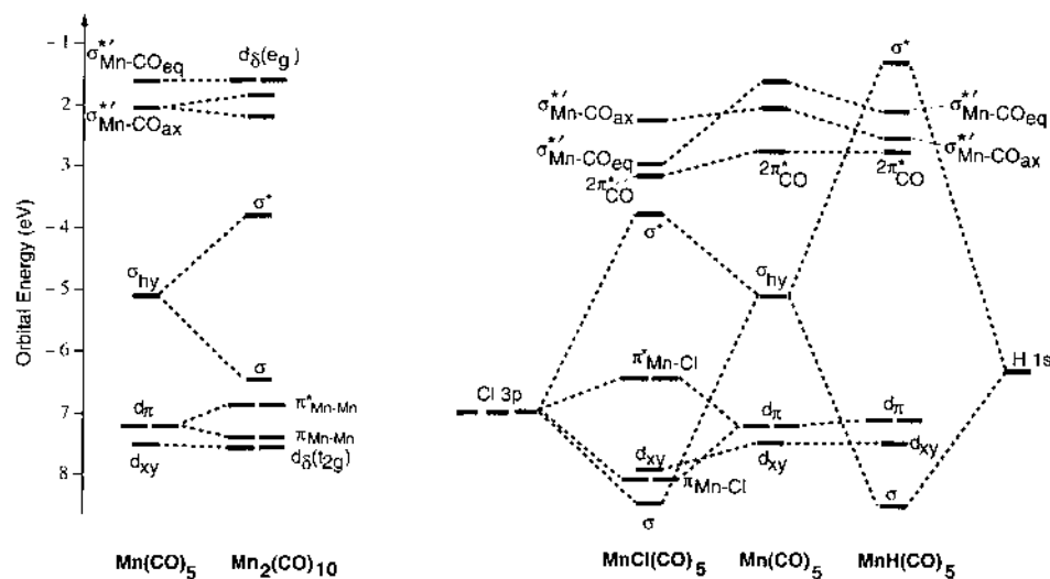
Fig. 4. Orbital interaction diagram for the formation of \text{Mn}(\text{CO})_5\text{L} , where \text{L} = \text{Mn}(\text{CO})_5 , \text{Cl} or \text{H} . The \text{Cl } 3p level is not at the energy calculated in the neutral atom but is positioned so as to suggest correctly the composition of the orbitals.
