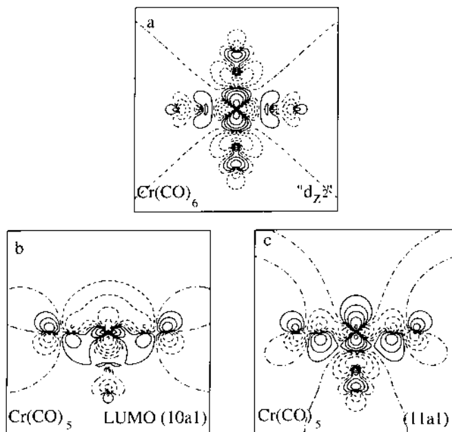
Fig. 3. (a) Orbital contour plot of the virtual e_g^* (“ d_{z^2} ”) orbital of \text{Cr}(\text{CO})_6 . Contour values: \pm 0.5 , \pm 0.2 , \pm 0.1 , \pm 0.05 , \pm 0.02 and 0.0 ( e \text{ bohr}^{-1} ) 1/2 . (b) Orbital contour plot of the a_1 LUMO of \text{Cr}(\text{CO})_5 , which is similar to the 10a_1 SOMO of \text{Mn}(\text{CO})_5 . (c) Orbital contour plot of the 11a_1 \sigma' orbital of \text{Cr}(\text{CO})_5 (similar to 11a_1 of \text{Mn}(\text{CO})_5 ).
